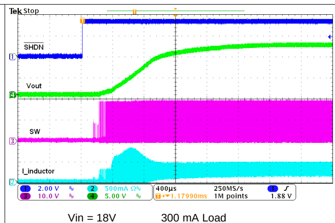
Figure 12. 12 V Output Start-Up Waveform
