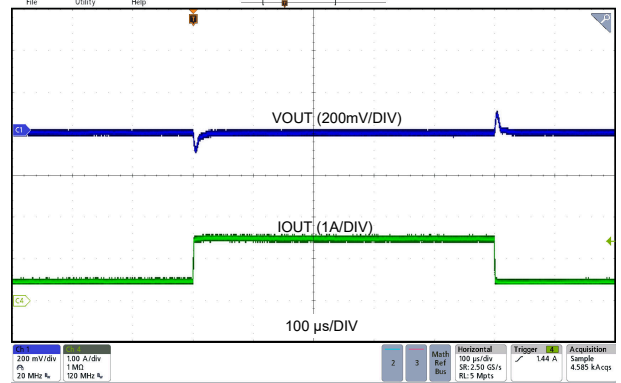
LMQ66430MC3 V_{OUT} = 3.3\text{ V} 2.2 MHz (Auto) 0.5 A to 1.5 A, 1 A / \mu s Fixed
