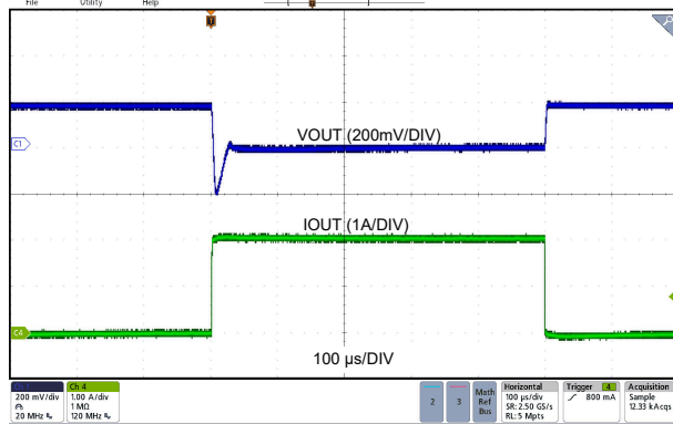
LMQ66430MC3 V_{OUT} = 3.3\text{ V} 2.2 MHz (Auto) 0 A to 2 A, 1 A / \mu s Fixed
