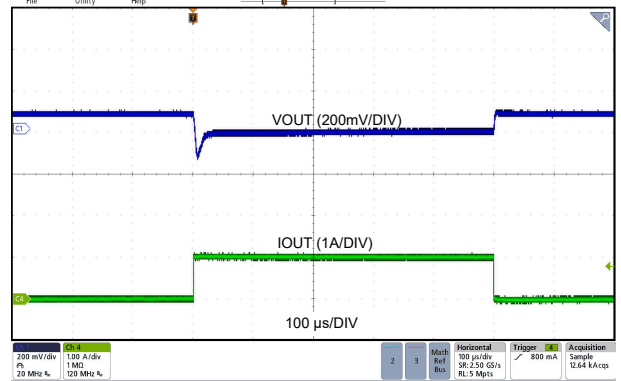
LMQ66430MC3 V_{OUT} = 3.3\text{ V} 2.2 MHz (Auto) 0 A to 1 A, 1 A / \mu s Fixed
