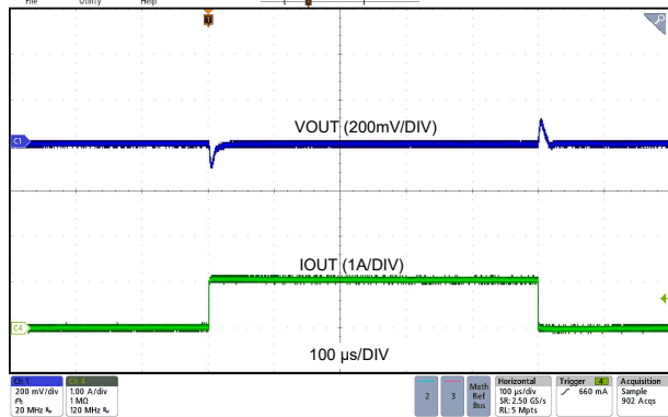
LMQ66430MC3 V_{OUT} = 3.3\text{ V} 2.2 MHz (FPWM) 0 A to 1 A, 1 A / \mu s Fixed
