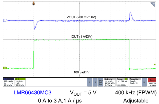
Figure 8-30. Load Transient
