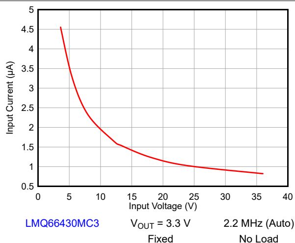
Figure 8-8. Input Switching Current vs Input Voltage
