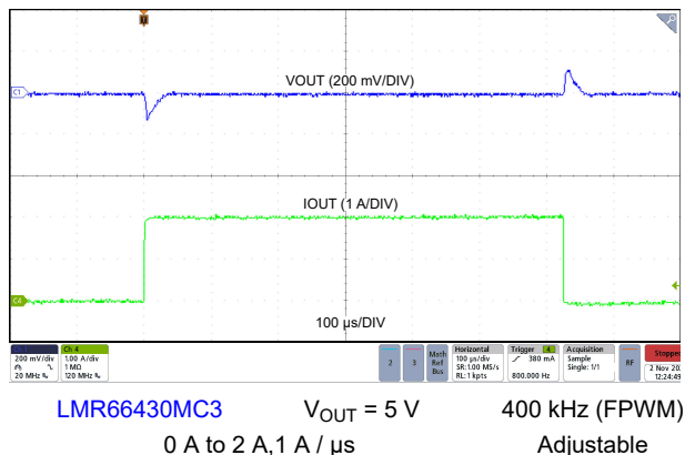
Figure 8-31. Load Transient
