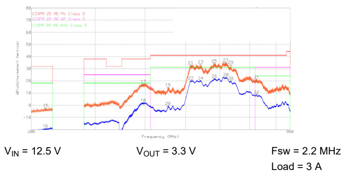
Figure 8-24. CISPR 25 Class 5 Radiated EMI, Log Antenna, Vertical Polarization, 300 MHz - 960 MHz Orange: Peak Detect, Blue: Average Detect
