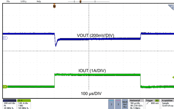
LMQ66430MC3 V_{OUT} = 3.3\text{ V} 2.2 MHz (Auto) 0 A to 1 A, 1 A / \mu\text{s} Fixed
