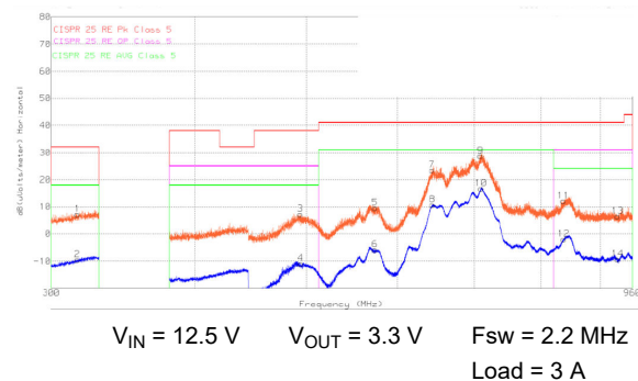
Figure 8-23. CISPR 25 Class 5 Radiated EMI, Log Antenna, Horizontal Polarization, 300 MHz - 960 MHz Orange: Peak Detect, Blue: Average Detect
