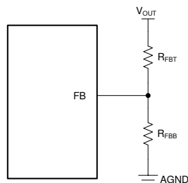
Figure 7-8. Setting Output Voltage for Adjustable Output Variant
