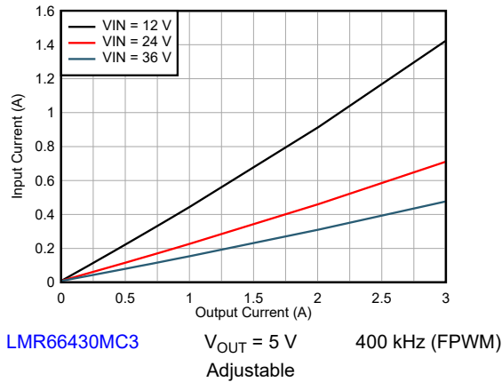
Figure 8-29. Input Current vs Load Current
