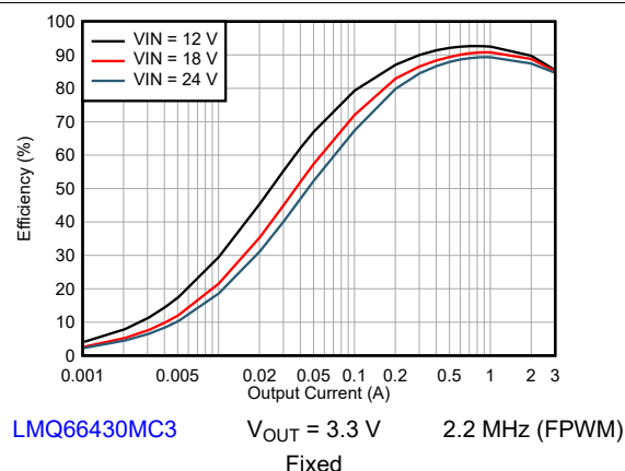
Figure 8-5. Efficiency
