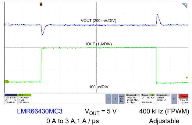
Figure 8-30. Load Transient
