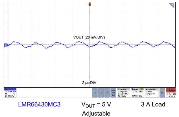
Figure 8-32. Output Voltage Ripple
