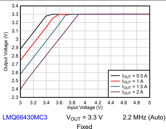
Figure 8-6. Dropout
