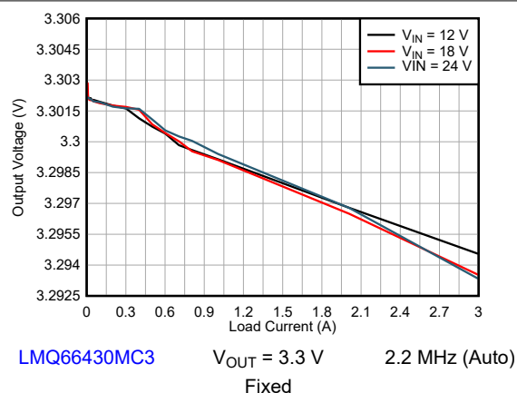
Figure 8-7. Line and Load Regulation
