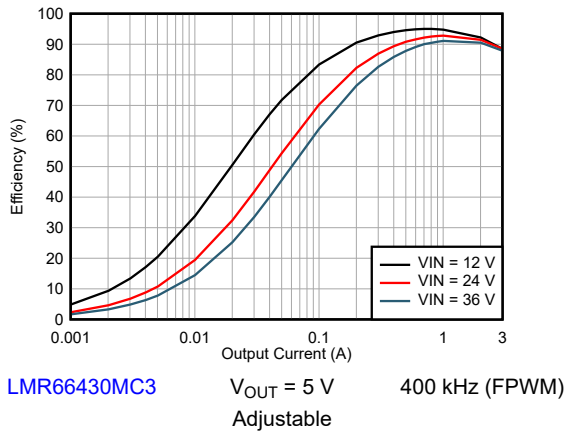
Figure 8-27. Efficiency
