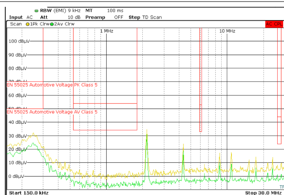
V_{IN} = 12.5\text{ V} V_{OUT} = 3.3\text{ V} Fsw = 2.2 MHz Load = 3 A
