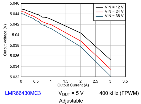
Figure 8-28. Line and Load Regulation
