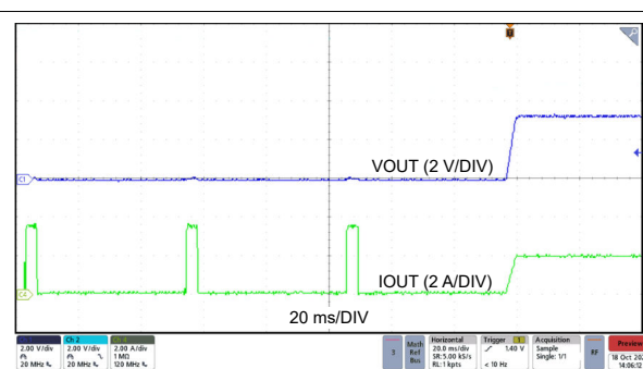
Figure 7-14. Hiccup Exit
