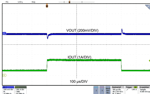
LMQ66430MC3 V_{OUT} = 3.3\text{ V} 2.2 MHz (Auto) 0.5 A to 1.5 A, 1 A / \mu\text{s} Fixed
