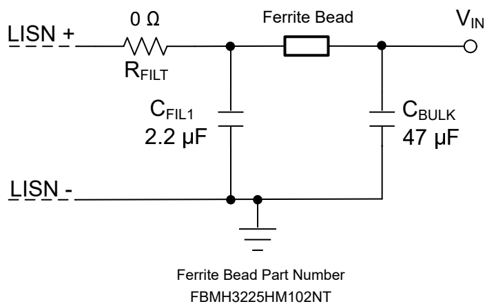
Figure 8-25. Typical Input EMI Filter
