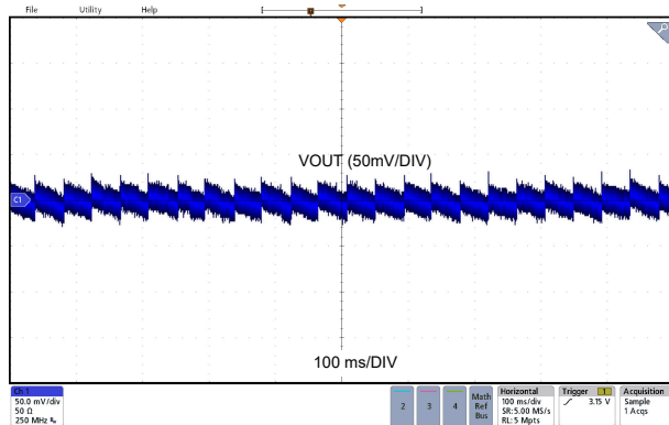
LMQ66430MC3 V_{OUT} = 3.3\text{ V} No Load Fixed
