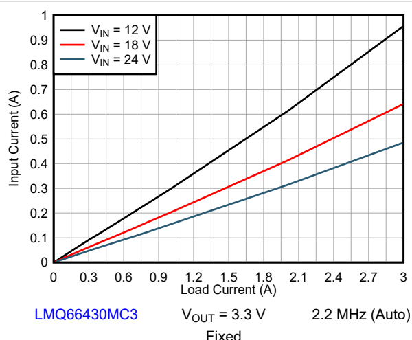
Figure 8-9. Input Current vs Load Current
