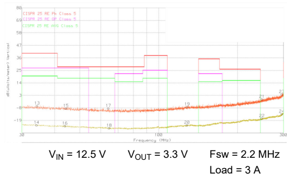
Figure 8-22. CISPR 25 Class 5 Radiated EMI, Biconical Antenna, Vertical Polarization, 30 MHz - 300 MHz Orange: Peak Detect, Yellow: Average Detect
