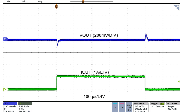
LMQ66430MC3 V_{OUT} = 3.3\text{ V} 2.2 MHz (FPWM) 0 A to 1 A, 1 A / \mu\text{s} Fixed
