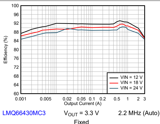
Figure 8-4. Efficiency
