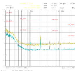
Conducted EMI: V_{\text{OUT}} = 5\text{ V} , I_{\text{OUT}} = 4\text{ A}
