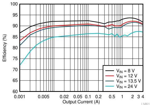
Figure 9-5. LMQ62440-Q1 Efficiency
