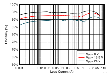
Efficiency: V_{\text{OUT}} = 5\text{ V} , F_{\text{SW}} = 2.1\text{ MHz}
