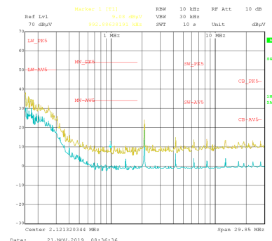
F_{SW} = 2100\text{ kHz} V_{OUT} = 5\text{ V} I_{OUT} = 5\text{ A} Frequency Tested: 150 kHz to 30 MHz
