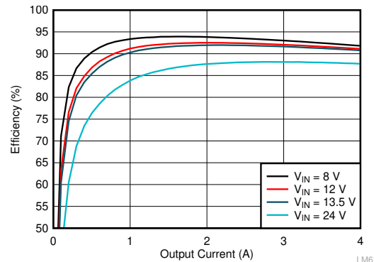
Figure 9-6. LMQ62440-Q1 Efficiency
