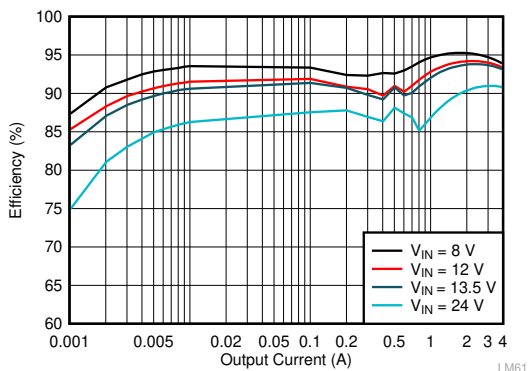
Figure 9-5. LMQ62440-Q1 Efficiency
