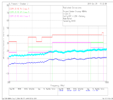
V_{OUT} = 5\text{ V} F_{SW} = 400\text{ kHz} I_{OUT} = 5\text{ A} Frequency Tested: 300 MHz to 1 GHz
