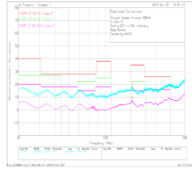
V_{OUT} = 5\text{ V} F_{SW} = 400\text{ kHz} I_{OUT} = 5\text{ A} Frequency Tested: 30 MHz to 300 MHz
