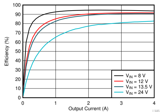
Figure 9-6. LMQ62440-Q1 Efficiency
