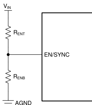
Figure 9-1. V_{IN} SYNC Using the EN pin
