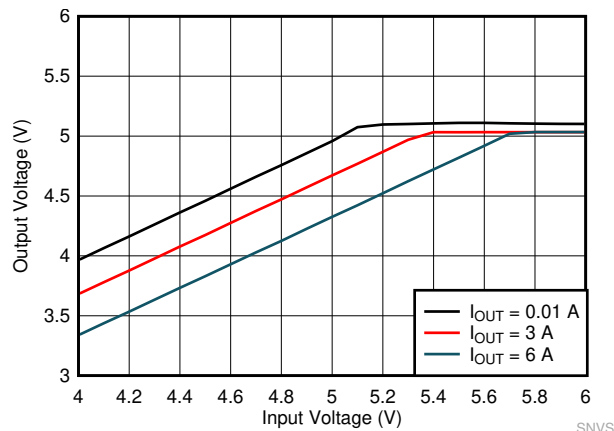
Figure 10-23. LMQ61460-Q1 Dropout Curve
