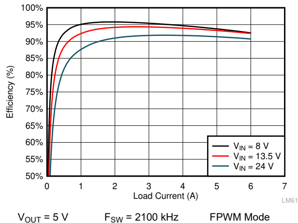
Figure 10-12. LMQ61460-Q1 Efficiency
