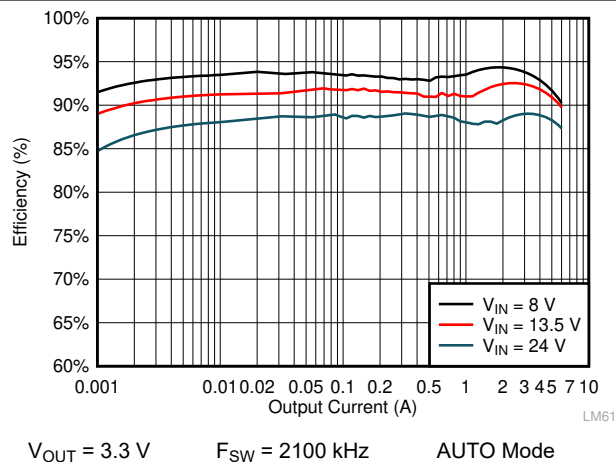
Figure 10-7. LMQ61460-Q1 Efficiency
