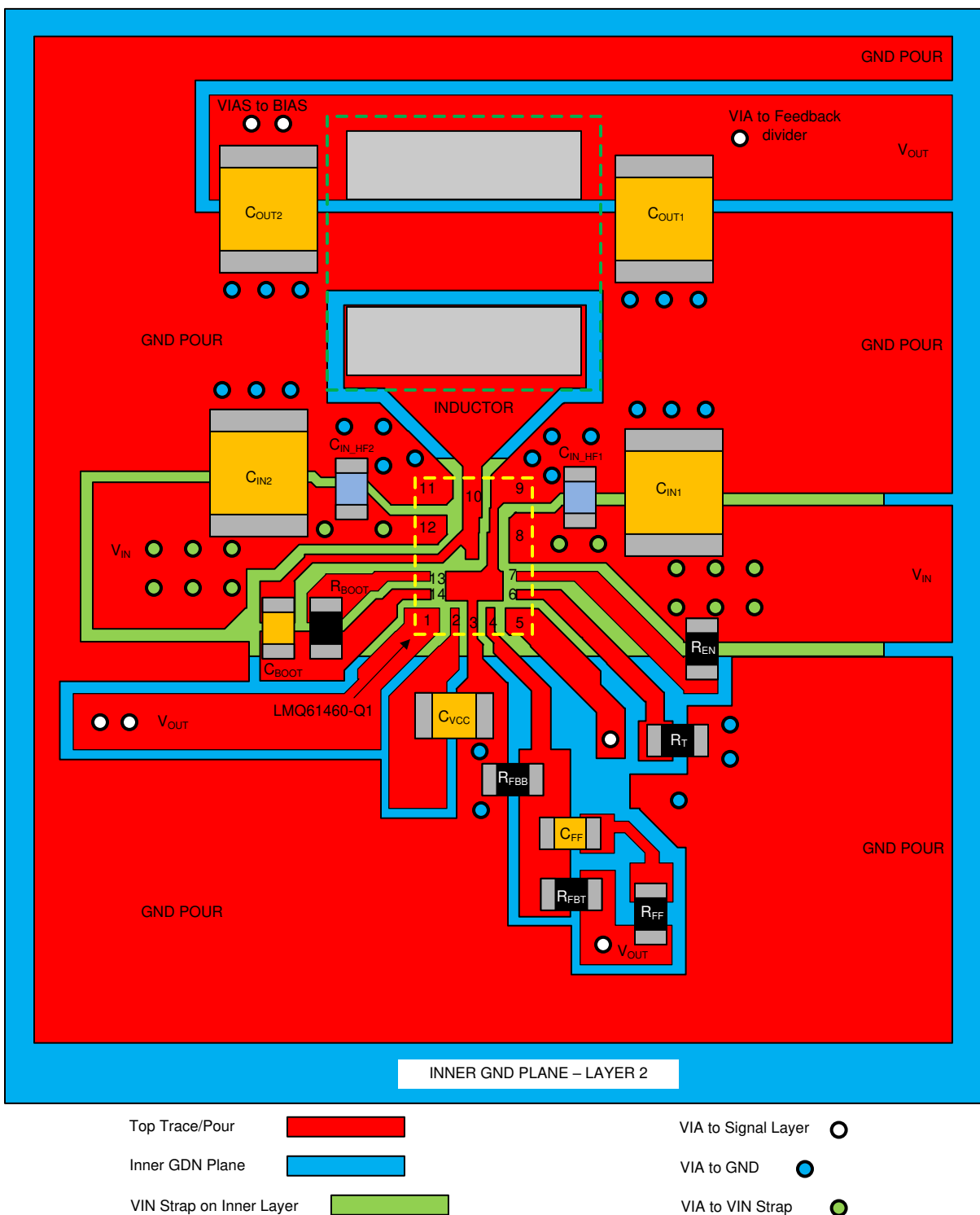
Figure 12-2. Layout Example
