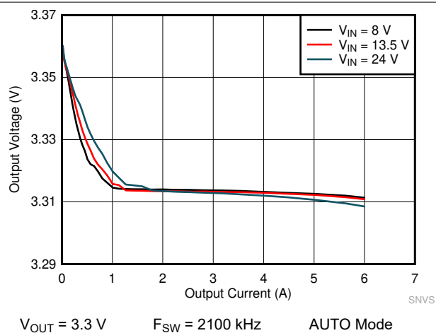
Figure 10-15. LMQ61460-Q1 Load and Line Regulation
