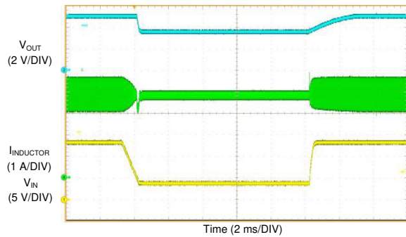
Figure 10-35. LMQ61460-Q1 Short Circuit Recovery
