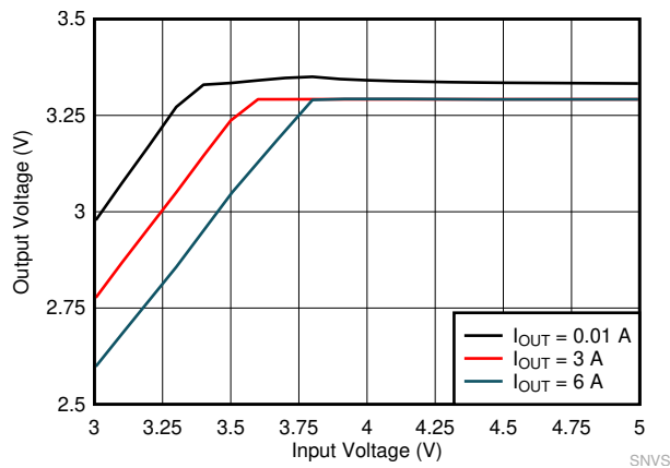
Figure 10-19. LMQ61460-Q1 Load and Line Regulation
