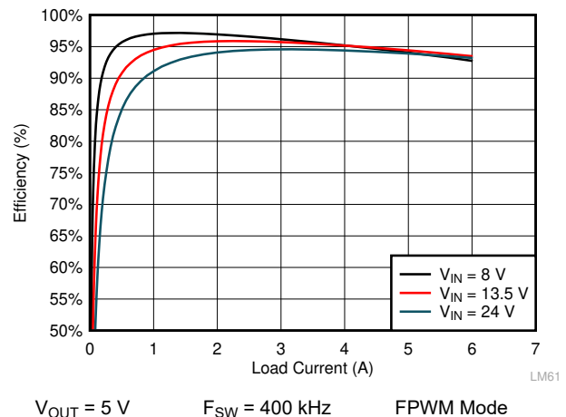
Figure 10-10. LMQ61460-Q1 Efficiency
