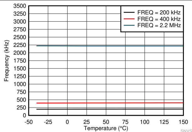
Figure 8-5. Switching Frequency
