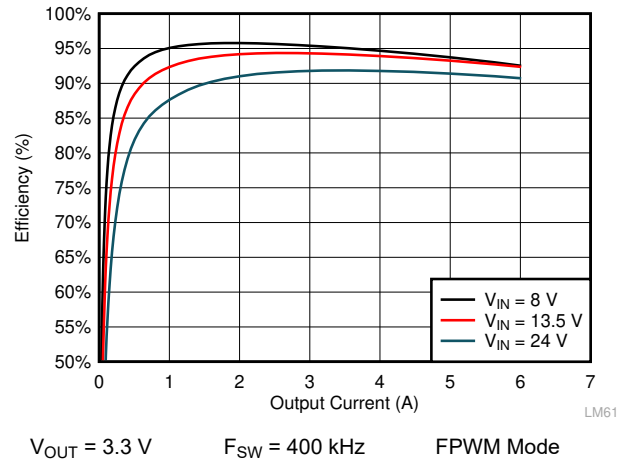
Figure 10-6. LMQ61460-Q1 Efficiency
