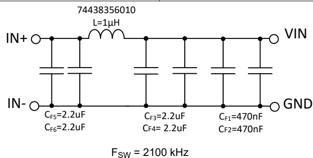
Figure 10-61. Recommended Input EMI Filter
