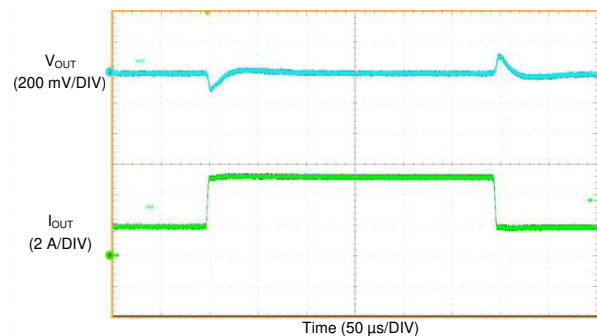
Figure 10-38. LMQ61460-Q1 Load Transient
