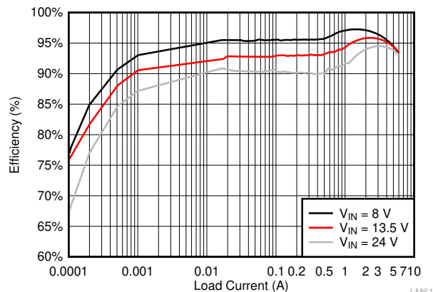
Efficiency: V_{OUT} = 5\text{ V} , F_{SW} = 400\text{ kHz}
