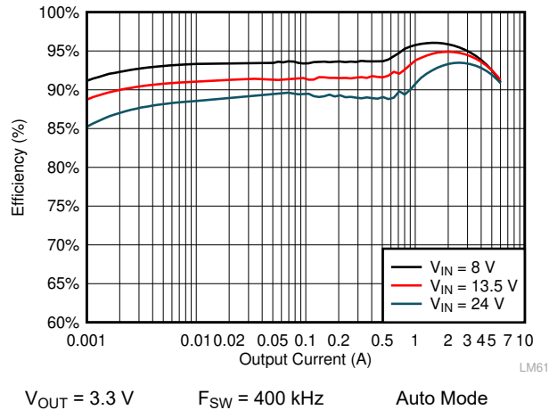
Figure 10-5. LMQ61460-Q1 Efficiency
