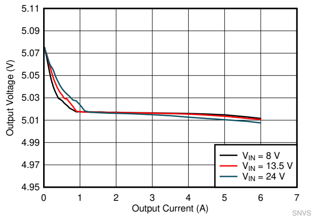
Figure 10-17. LMQ61460-Q1 Load and Line Regulation
