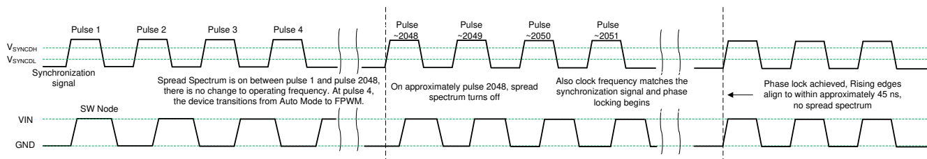
Figure 9-5. Synchronization Process
