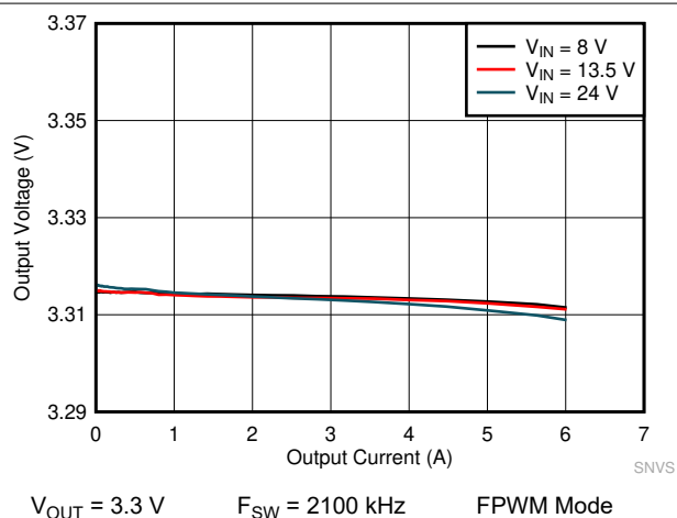
Figure 10-16. LMQ61460-Q1 Load and Line Regulation
