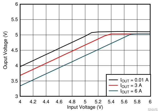
Figure 10-24. LMQ61460-Q1 Dropout Curve
