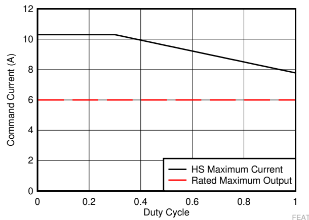
Figure 9-12. Maximum Current Allowed Through the HS FET - Function of Duty Cycle for LMQ61460-Q1
