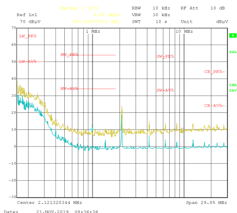
Conducted EMI: V_{OUT} = 5\text{ V} , I_{OUT} = 4\text{ A}
