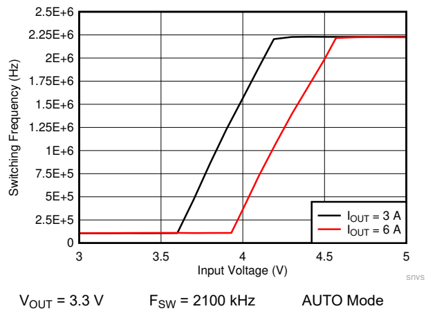
Figure 10-26. LMQ61460-Q1 Frequency Dropout Curve
