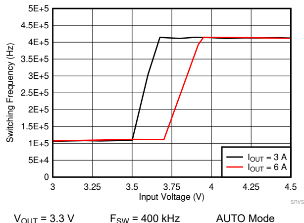
Figure 10-25. LMQ61460-Q1 Frequency Dropout Curve
