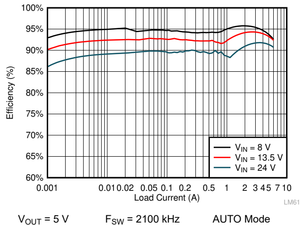
Figure 10-11. LMQ61460-Q1 Efficiency
