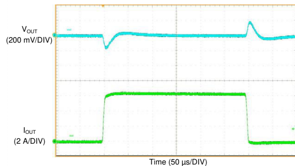
Figure 10-43. LMQ61460-Q1 Load Transient
