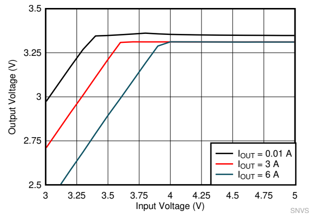
Figure 10-20. LMQ61460-Q1 Load and Line Regulation
