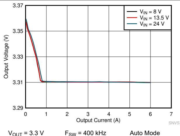
Figure 10-13. LMQ61460-Q1 Load and Line Regulation
