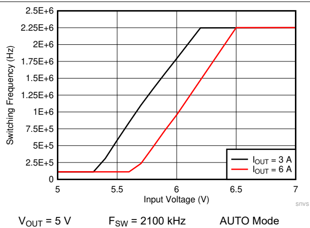
Figure 10-28. LMQ61460-Q1 Frequency Dropout Curve
