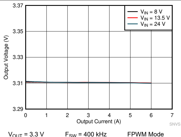
Figure 10-14. LMQ61460-Q1 Load and Line Regulation
