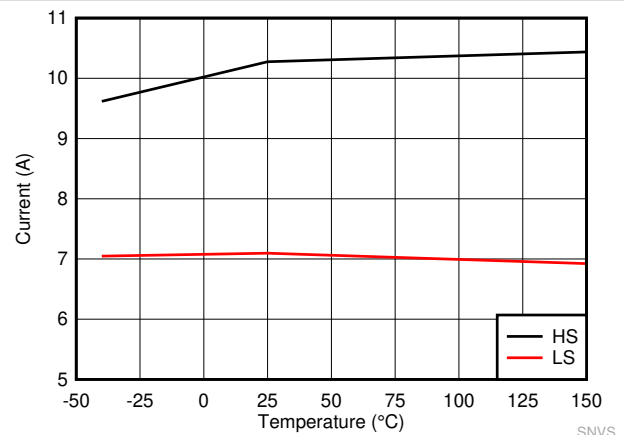
Figure 8-4. LMQ61460-Q1 High-Side and Low-Side Current Limits
