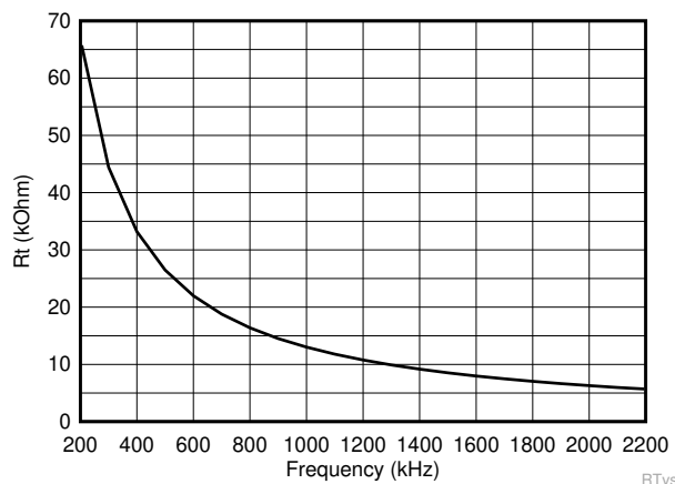
Figure 9-4. Setting Clock Frequency
