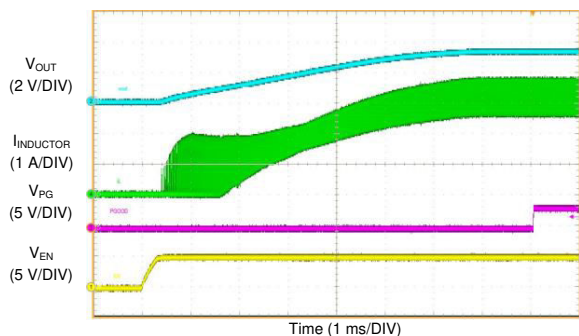
Figure 10-31. LMQ61460-Q1 Start-up with 50-mA Load
