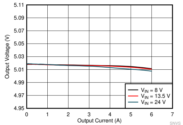
Figure 10-18. LMQ61460-Q1 Load and Line Regulation
