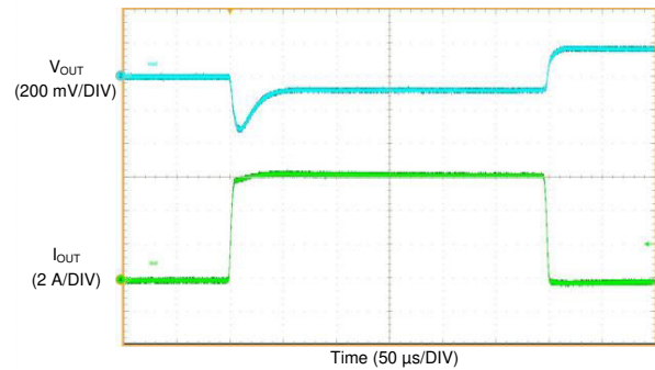
Figure 10-42. LMQ61460-Q1 Load Transient
