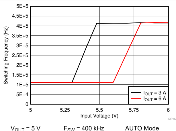
Figure 10-27. LMQ61460-Q1 Frequency Dropout Curve
