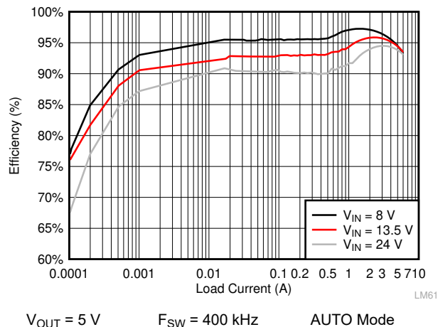
Figure 10-9. LMQ61460-Q1 Efficiency
