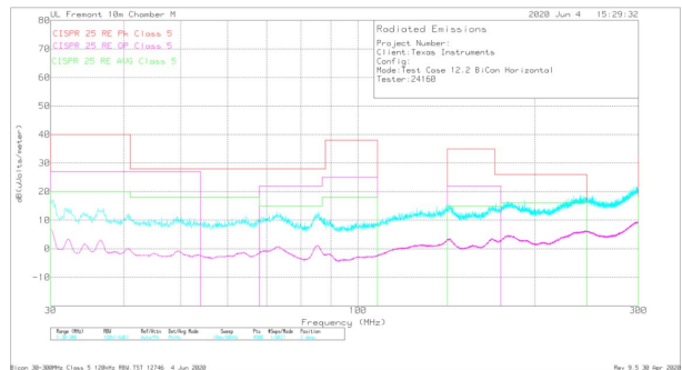
Figure 10-56. Radiated EMI Red versus CISPR25 Limits
