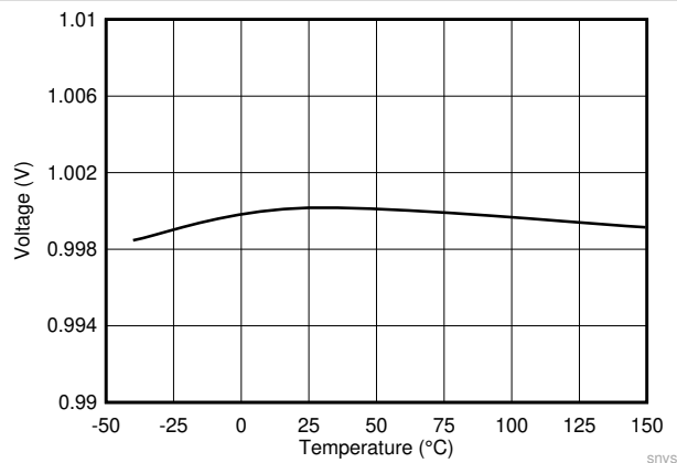
Figure 8-3. Feedback Voltage
