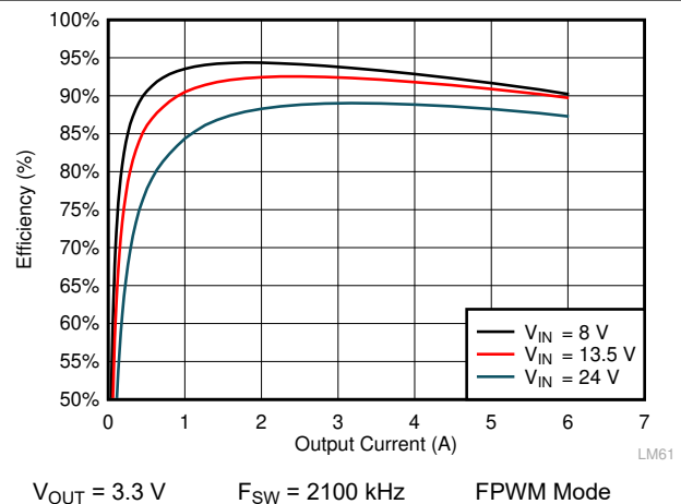
Figure 10-8. LMQ61460-Q1 Efficiency
