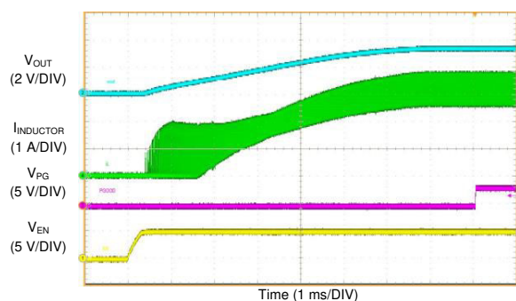
Figure 9-31. LMQ61460 Start-Up with 50-mA Load
