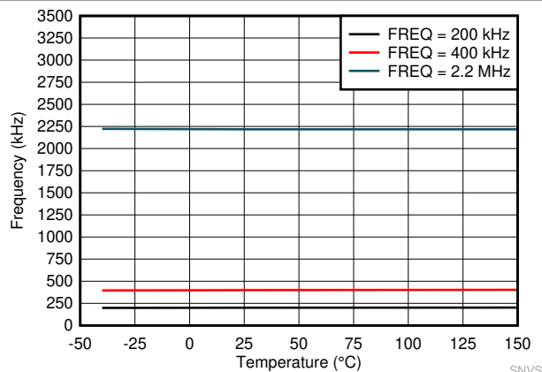
Figure 7-5. Switching Frequency
