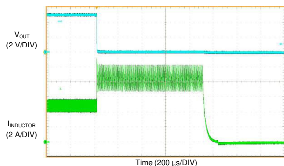
Figure 9-32. LMQ61460 Start-Up with 50-mA Load
