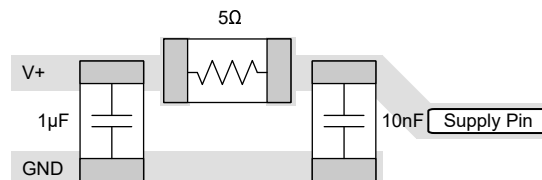
Figure 7-8. LMP7704-SP Supply Decoupling Capacitance Example Layout
