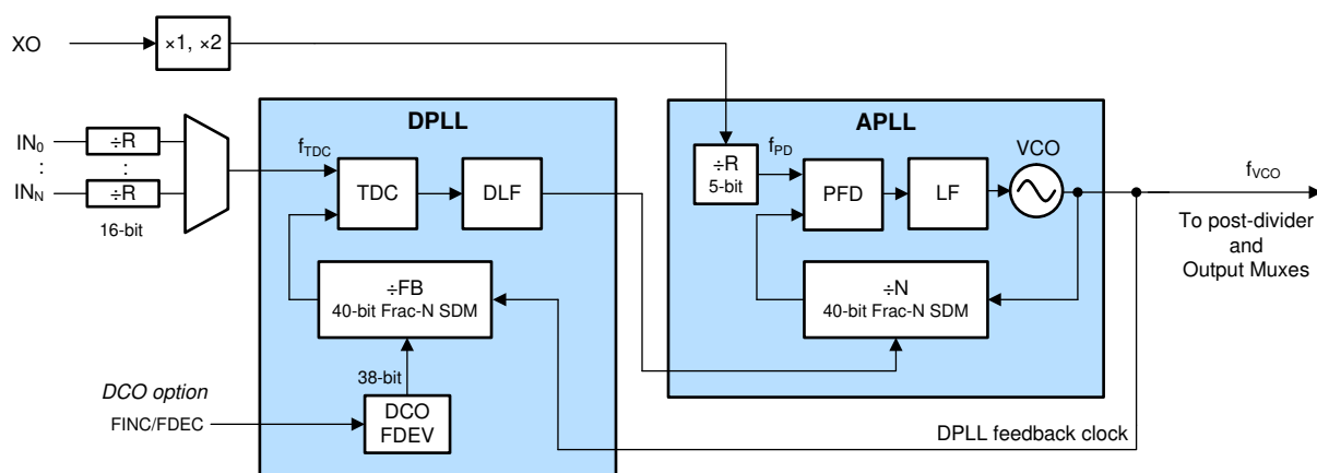
Figure 8-23. PLL Architecture
