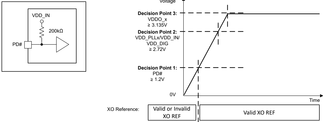
Figure 8-1. Recommendation for Power Up From a Single-Supply Rail
