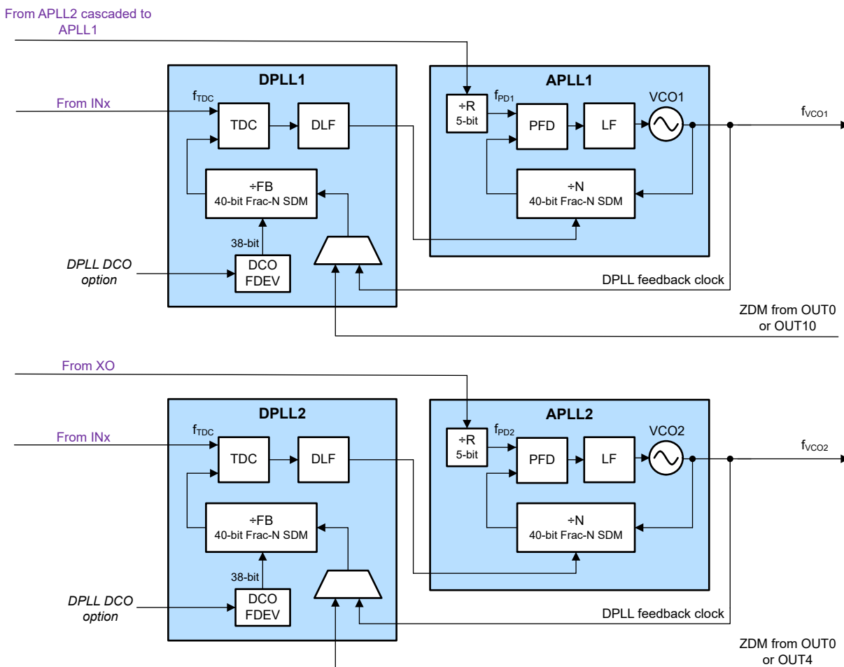
Figure 7-4. APLL Cascaded With DPLLs Enabled Example
