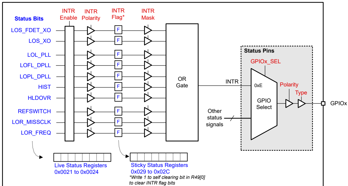
Figure 7-21. Status and Interrupt
