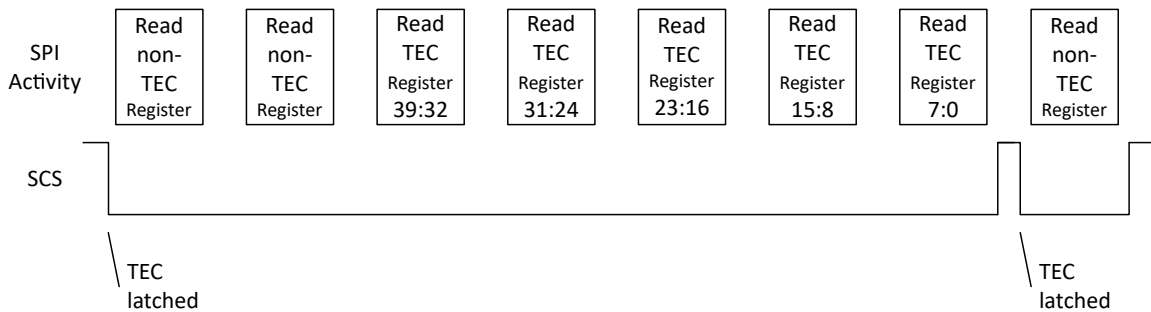
Figure 7-35. TEC Multibyte Read
