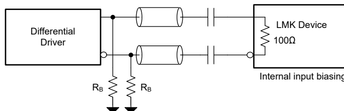
Figure 7-14. AC-Coupled Differential to Reference (INx)
