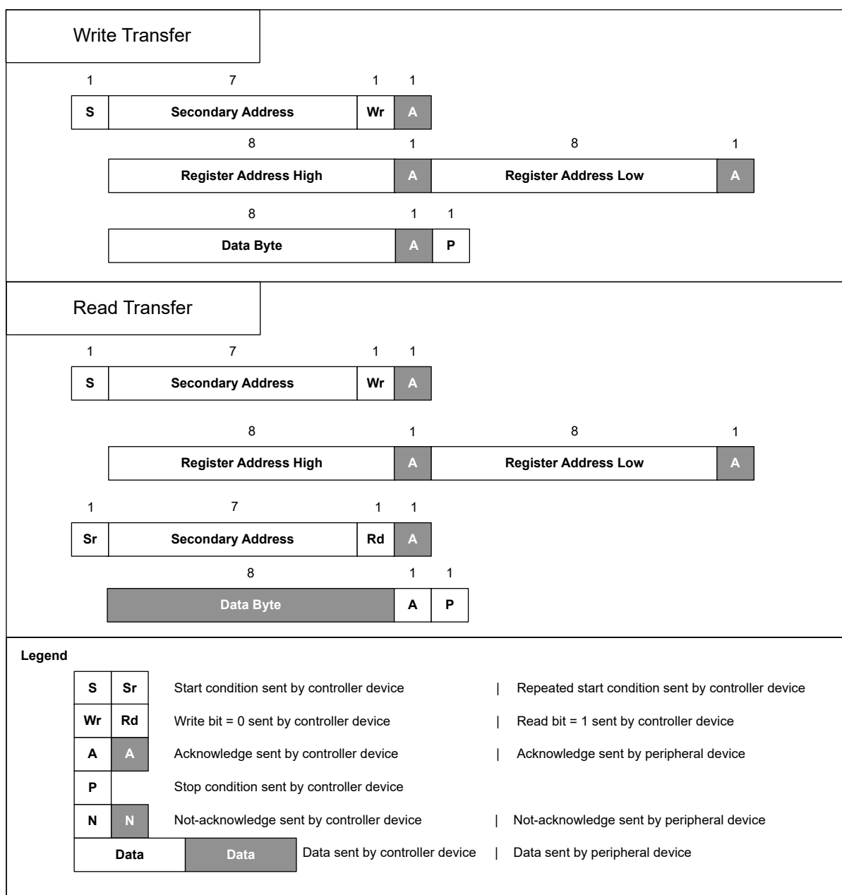
Figure 8-43. I 2 C Byte Write and Read Transfers
