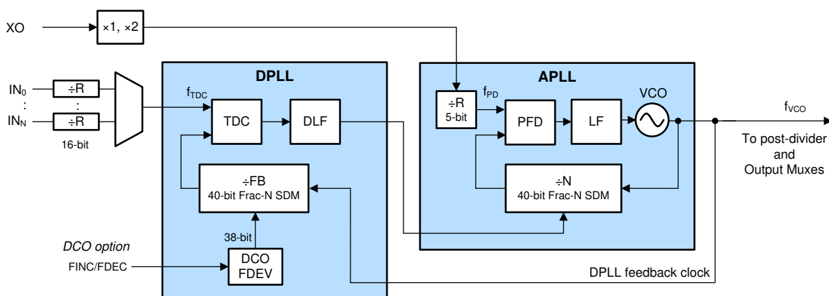
Figure 8-21. PLL Architecture
