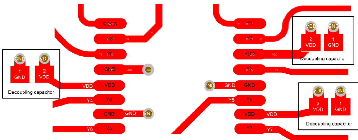
Figure 11-1. PCB Conceptual Layout
