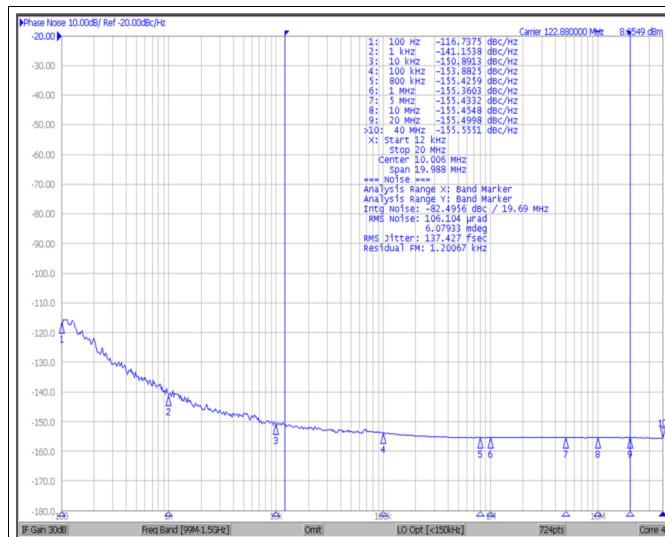
Figure 35. OSCout, 122.88 MHz, LVCOS (Norm/Inv) Normal Output Measured, Inverse 50-Ω Termination
