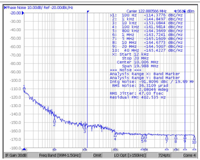
Figure 36. Direct VCXO Measurement Open-Loop, Holdover Mode Set
