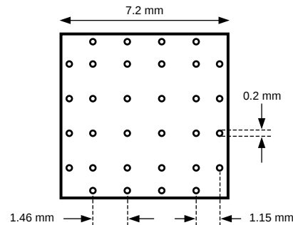
Figure 15. Recommended Land and Via Pattern
