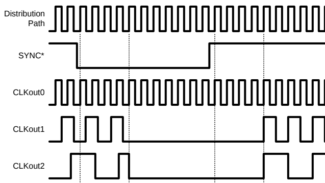
Figure 5-2. SYNC* Timing Diagram
