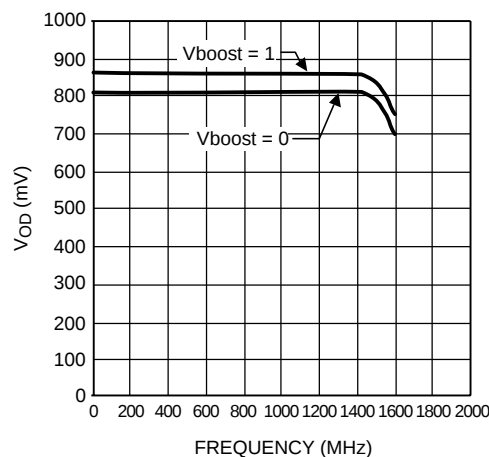
Figure 4-2. LVPECL Vod
