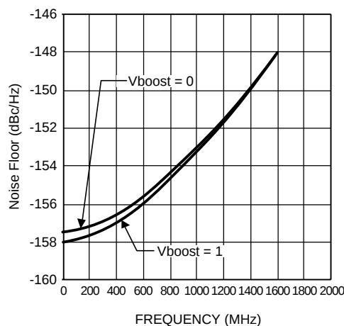
Figure 4-4. LVPECL Output Buffer Noise Floor
