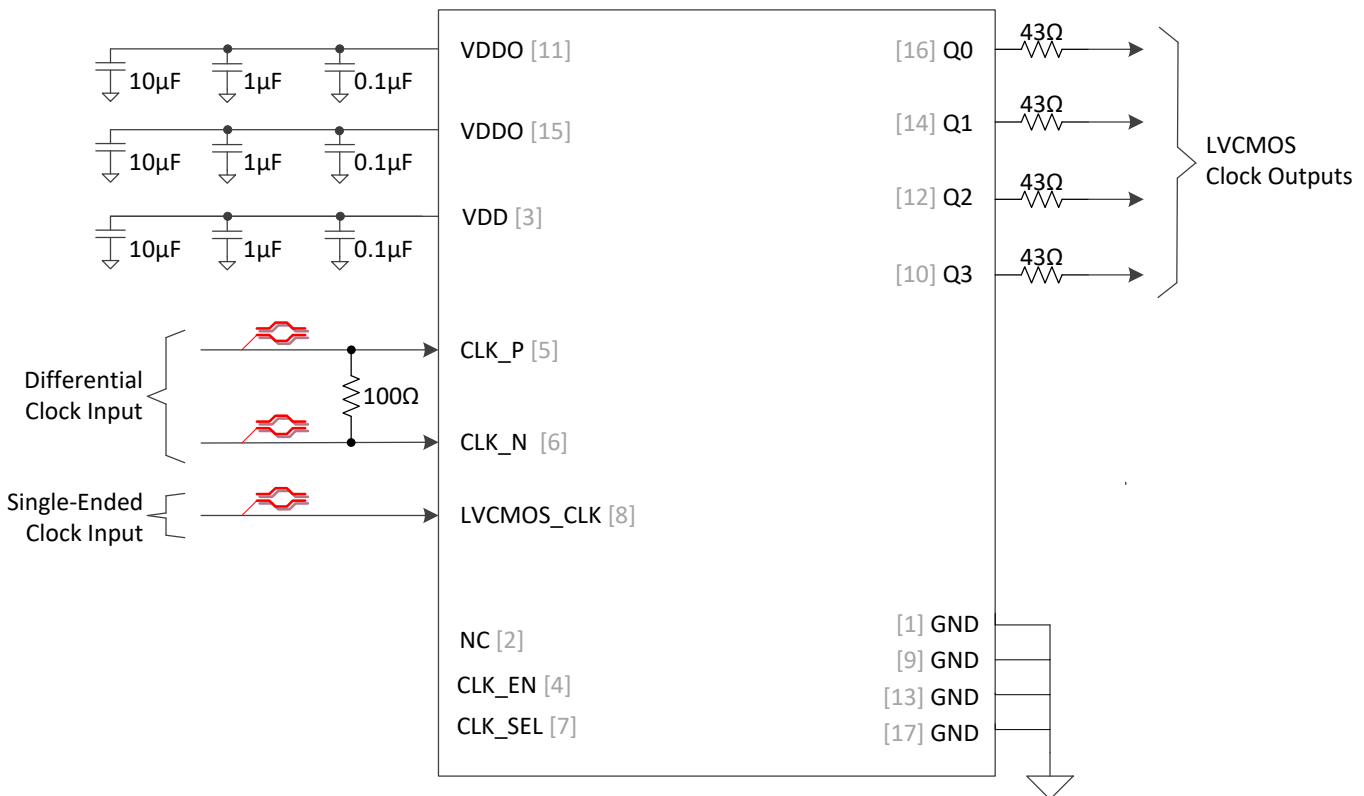
Figure 9. Typical Connection Diagram
