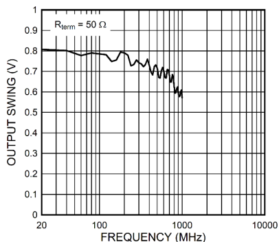
Figure 7-3. HCSL Output Swing ( V_{OD} ) vs Frequency
