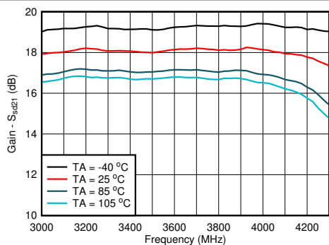
Figure 6-1. Gain vs Frequency and Temperature
