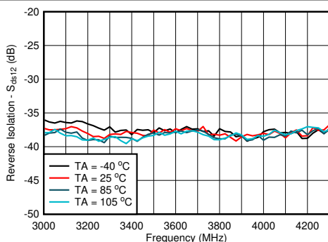
Figure 6-5. Reverse Isolation vs Frequency
