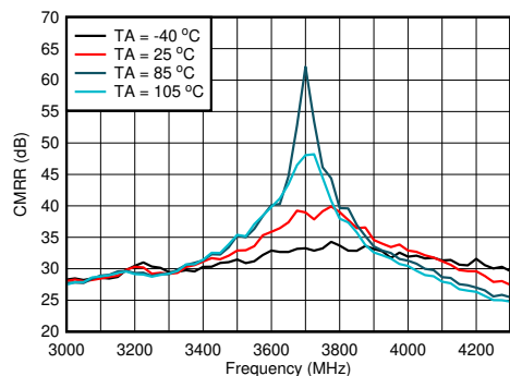
Figure 6-13. Common-mode Rejection Ratio vs Frequency
