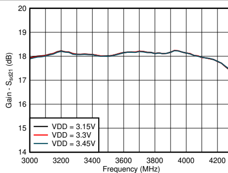
Figure 6-2. Gain vs Frequency and Supply Voltage
