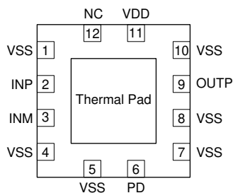
Figure 5-1. RRL Package 12-Pin WQFN Top View
