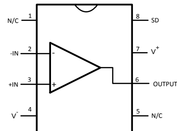
SOIC-8 (LMH6647) Package D08A Top View
