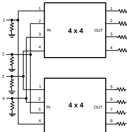
Figure 59. Output Expansion
