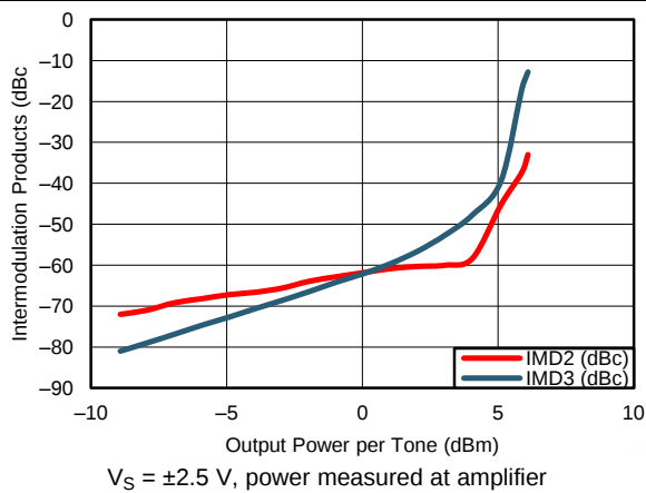
Figure 33. Intermodulation Distortion (f = 1000 MHz)
