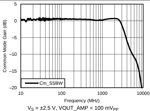
Figure 11. Common-Mode Frequency Response
