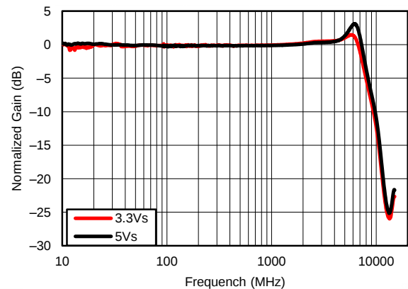
Figure 2. Frequency Response Differential Input
