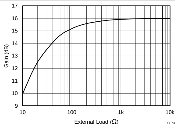
Figure 70. Net Gain versus Load Resistance
