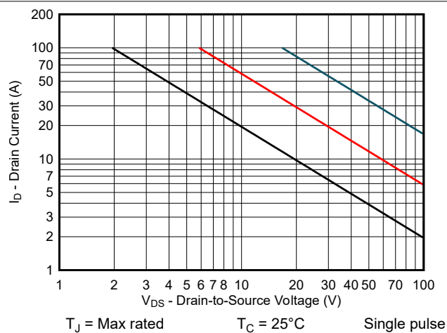
Figure 5-16. LMG3100R044 Safe Operating Area
