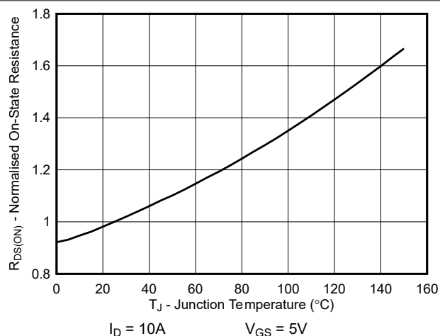
Figure 5-14. LMG3100R044 Normalized On-State Resistance vs Junction Temperature
