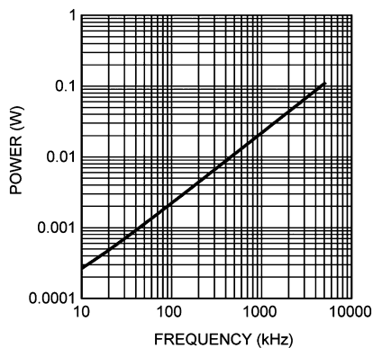
Figure 8-3. Forward Bias Power Loss of Bootstrap Diode V_{IN} = 50 V
