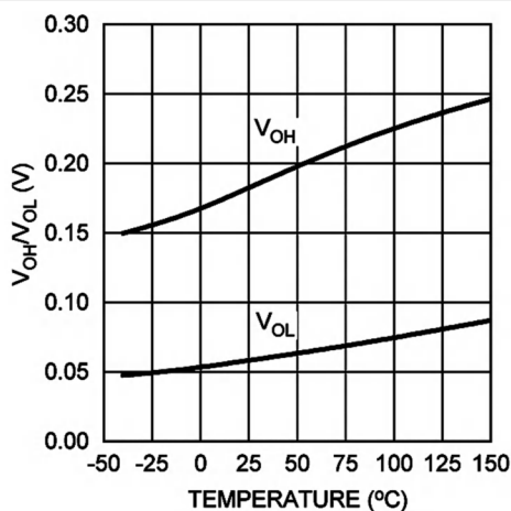
Figure 6-14. LO &amp; HO Gate Drive – High/Low Level Output Voltage vs Temperature
