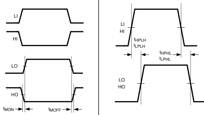
Figure 6-1. Timing Diagram
