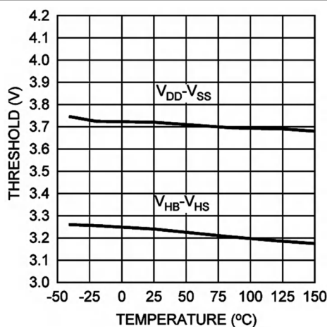
Figure 6-9. UVLO Falling Thresholds vs Temperature
