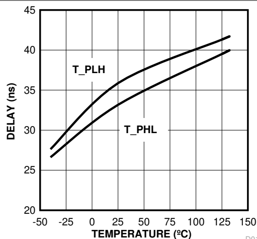
Figure 6-13. Propagation Delay vs Temperature
