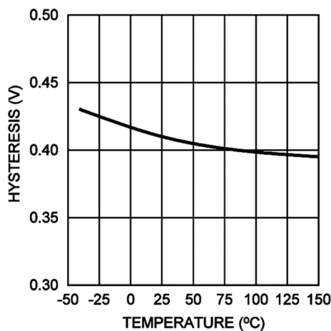
Figure 6-11. Input Threshold Hysteresis vs Temperature
