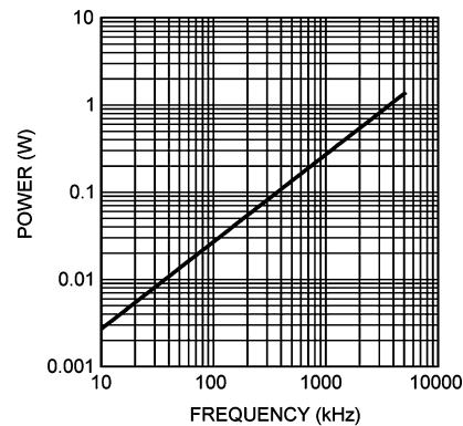
Figure 8-4. Reverse Recovery Power Loss of Bootstrap Diode V_{IN} = 50 V
