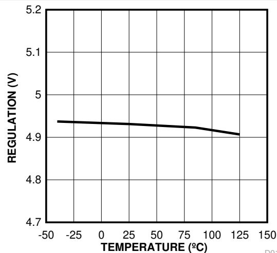
Figure 6-15. HB Regulation Voltage vs Temperature
