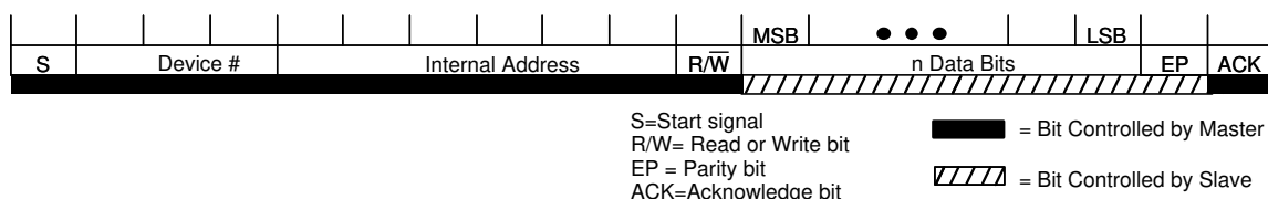
Figure 6-3. Read Transaction, master reads data from LM95010
