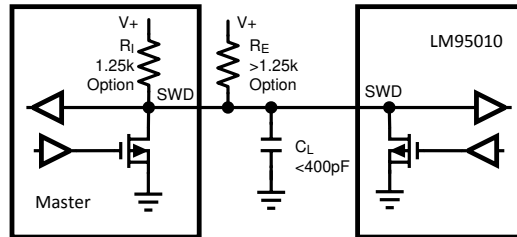
Figure 6-1. SensorPath SWD simplified schematic
