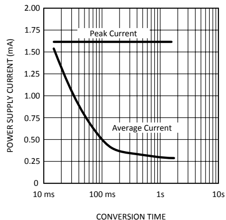
Figure 5-4. Conversion Rate Effect on Power Supply Current
