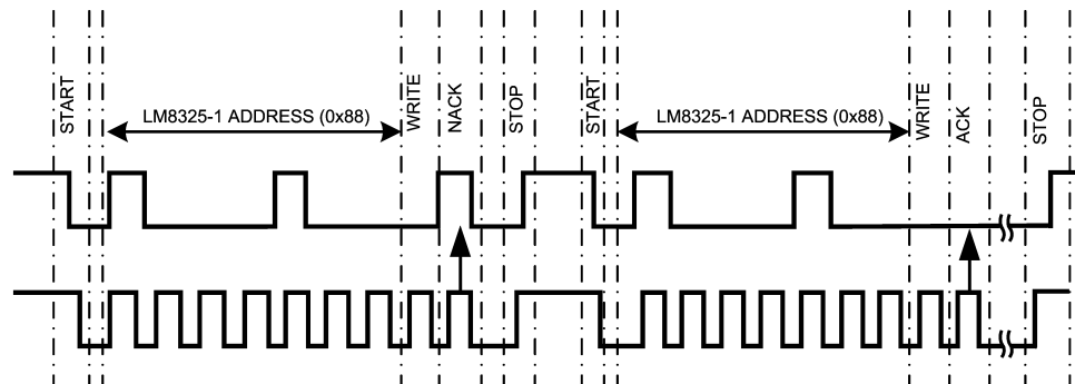
Figure 5. Host Starts Communication While LM8325-1 is in Sleep Mode
