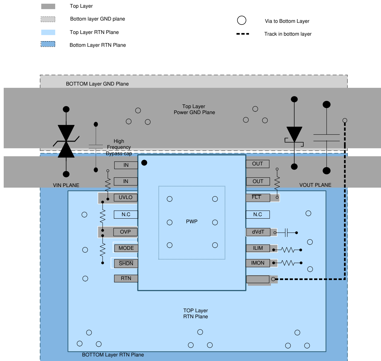
Figure 49. Typical PCB Layout Example With HTSSOP Package With a 2-Layer PCB
