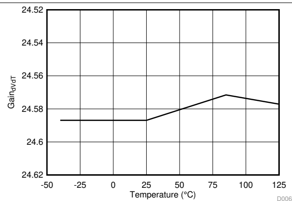
Figure 6. GAIN( dVdT ) vs Temperature
