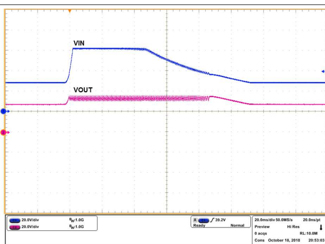
Figure 24. Programmable Overvoltage Clamp Response
