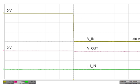
Figure 28. Reverse Input Supply Protection at -60 V
