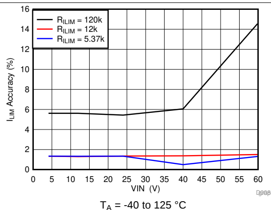
Figure 8. I_{LIM} Accuracy vs Supply Voltage
