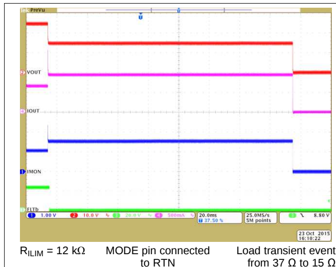
Figure 38. Look Ahead Overload Current Fault Indication
