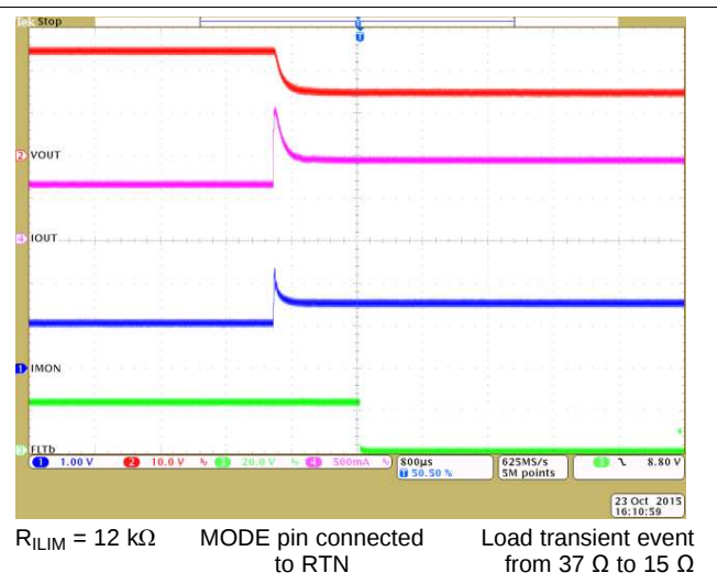
Figure 39. Output Turnoff Due to Thermal Shutdown With \overline{\text{FLT}} Asserted in Advance
