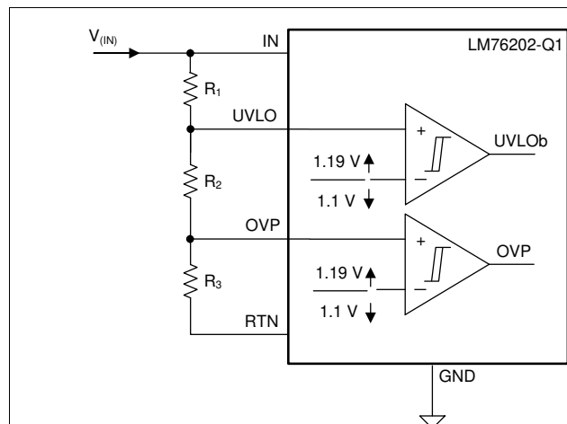
Figure 21. OVP Threshold Setting
