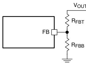
Figure 11. Output Voltage Setting
