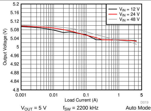
Figure 43. LM76003-Q1 Load and Line Regulation
