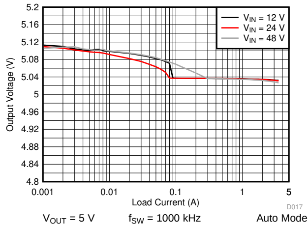
Figure 41. LM76003-Q1 Load and Line Regulation
