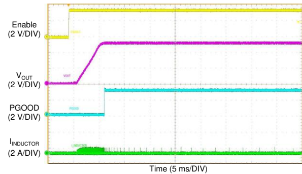
Figure 66. LM76003-Q1 Start-up Waveform
