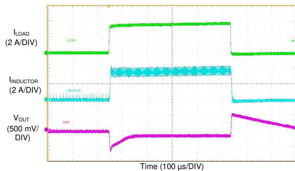
Figure 79. LM76003-Q1 Load Transient
