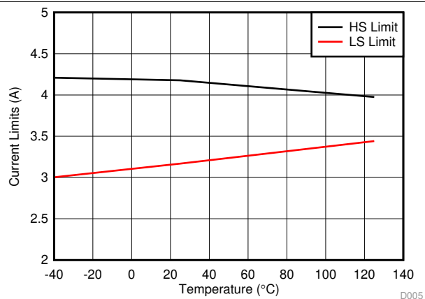
Figure 5. LM76002-Q1 High-Side and Low-Side Current Limits
