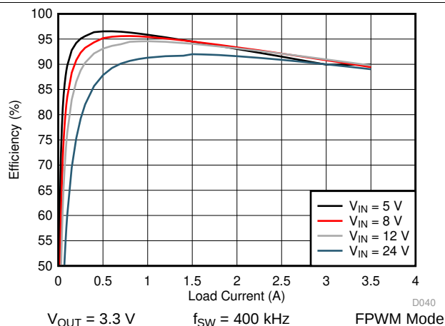
Figure 24. LM76003-Q1 Efficiency
