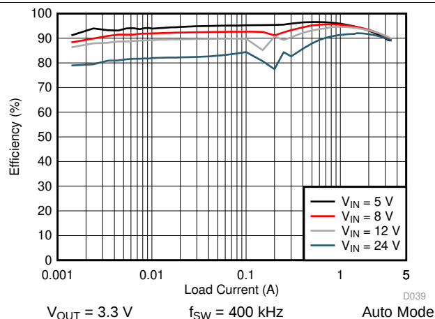
Figure 23. LM76003-Q1 Efficiency
