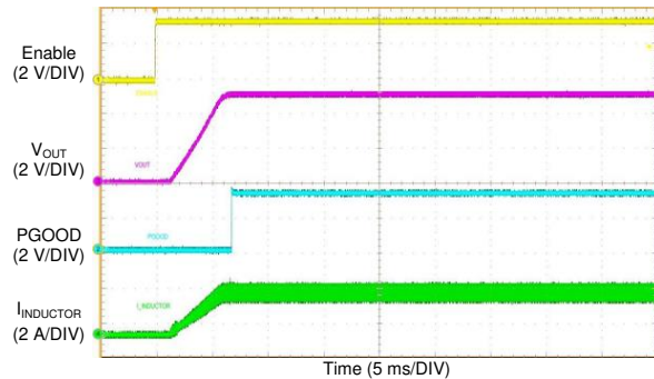
Figure 67. LM76003-Q1 Start-up Waveform
