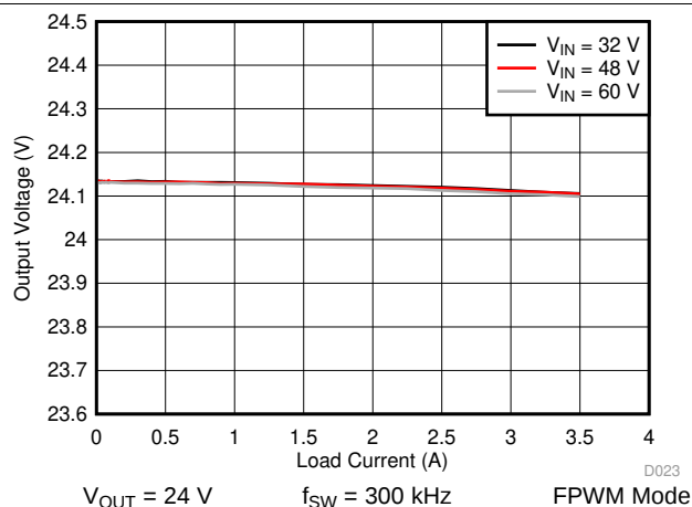
Figure 48. LM76003-Q1 Load and Line Regulation
