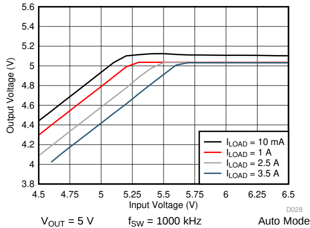
Figure 53. LM76003-Q1 Dropout Curve
