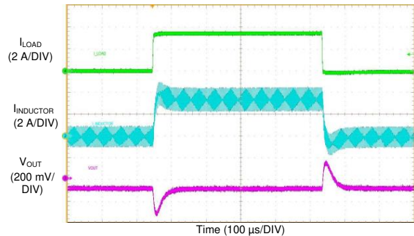
Figure 74. LM76003-Q1 Load Transient
