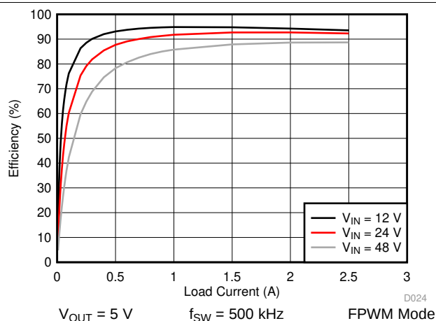
Figure 36. LM76002-Q1 Efficiency
