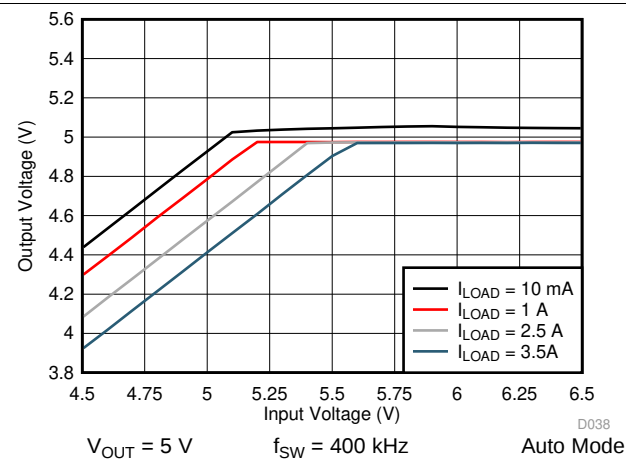
Figure 52. LM76003-Q1 Dropout Curve
