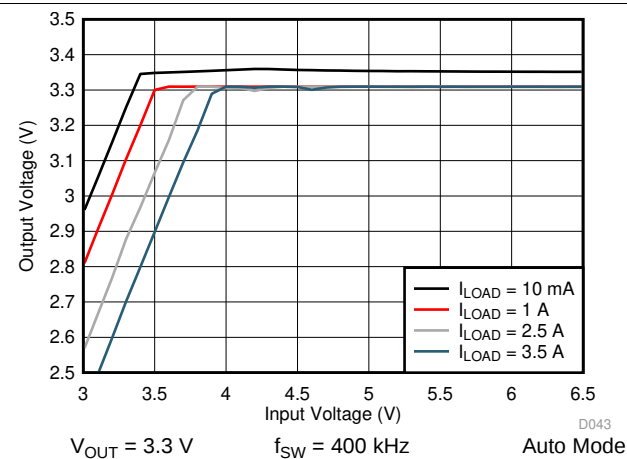
Figure 51. LM76003-Q1 Dropout Curve
