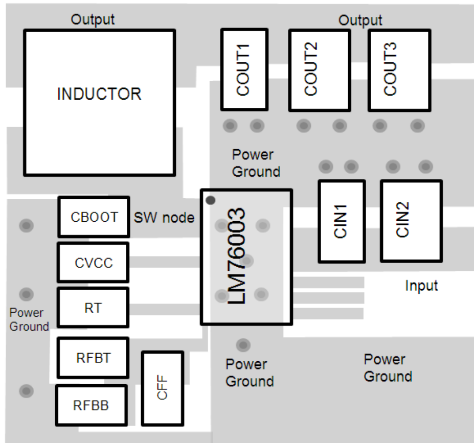
Figure 91. LM76002-Q1/LM76003-Q1 Layout
