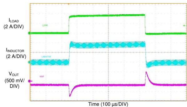
Figure 80. LM76003-Q1 Load Transient
