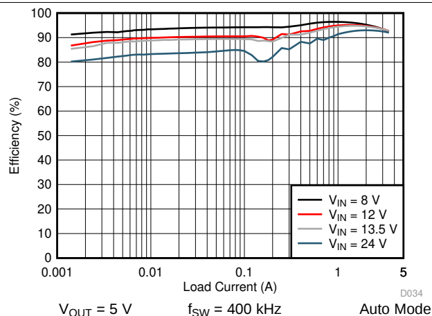
Figure 25. LM76003-Q1 Efficiency
