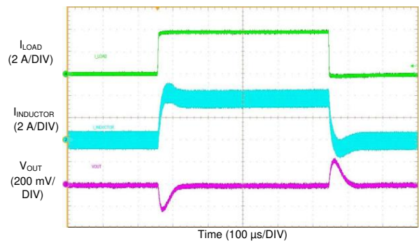
Figure 78. LM76003-Q1 Load Transient
