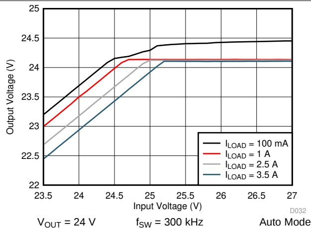
Figure 57. LM76003-Q1 Dropout Curve
