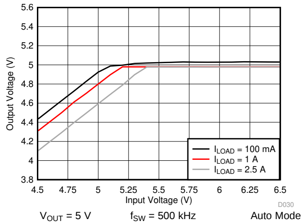
Figure 55. LM76002-Q1 Dropout Curve
