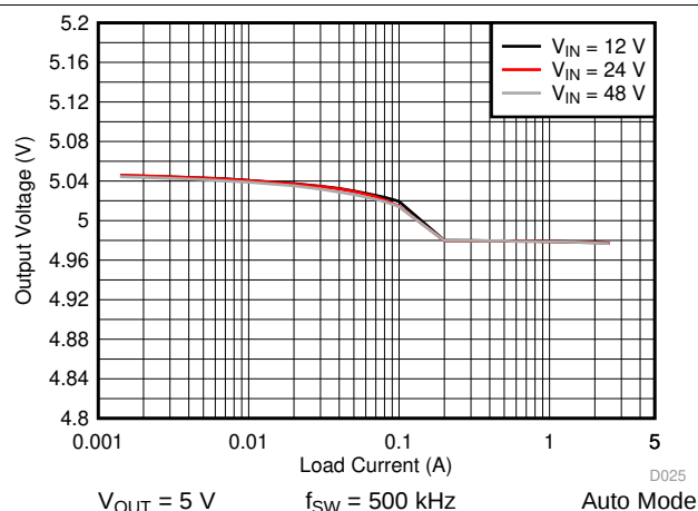
Figure 49. LM76002-Q1 Load and Line Regulation
