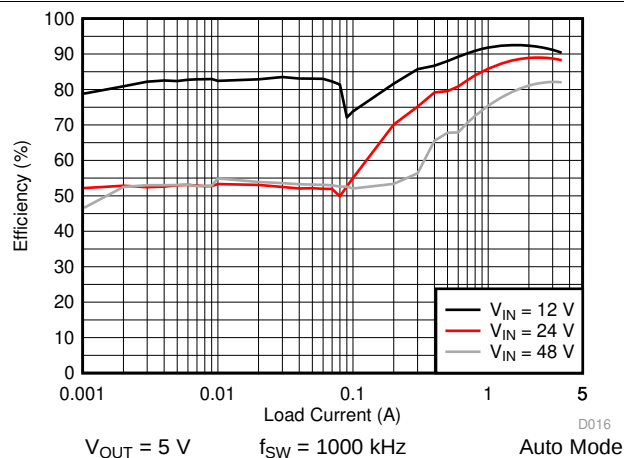
Figure 27. LM76003-Q1 Efficiency
