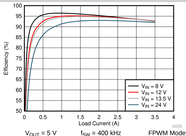
Figure 26. LM76003-Q1 Efficiency
