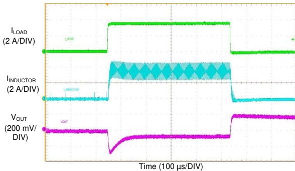
Figure 73. LM76003-Q1 Load Transient
