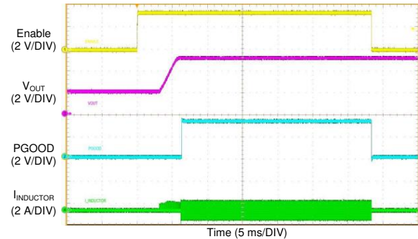
Figure 68. LM76002-Q1 Start-up Waveform
