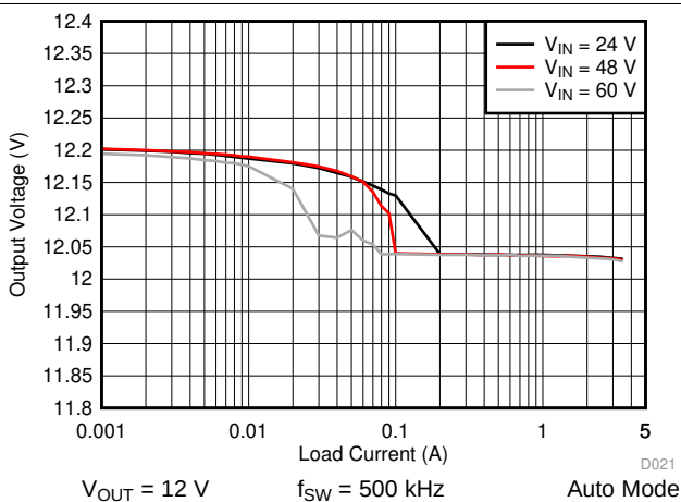
Figure 45. LM76003-Q1 Load and Line Regulation
