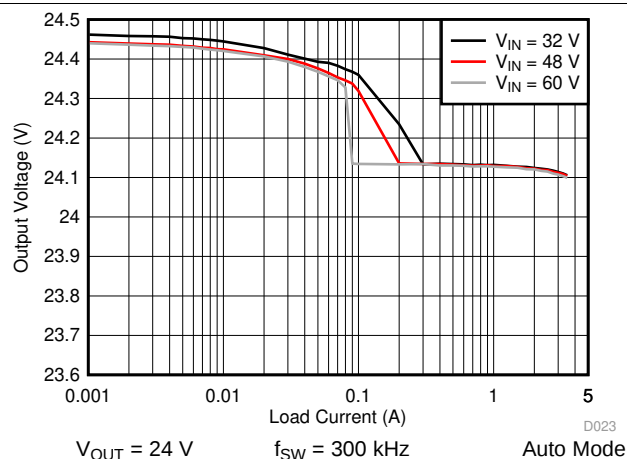
Figure 47. LM76003-Q1 Load and Line Regulation
