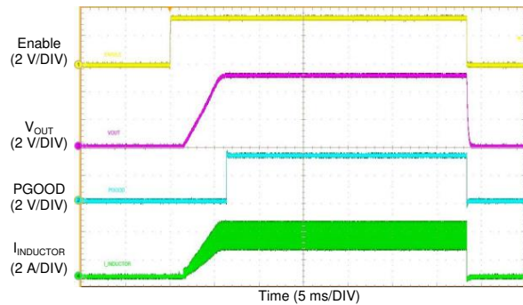
Figure 65. LM76003-Q1 Start-up Waveform
