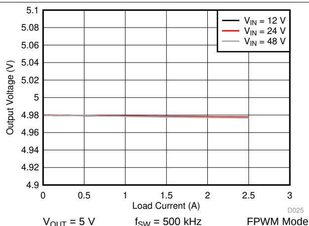
Figure 50. LM76002-Q1 Load and Line Regulation
