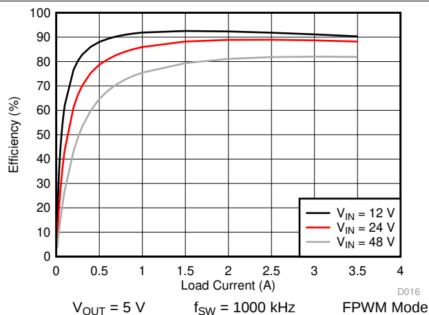
Figure 28. LM76003-Q1 Efficiency
