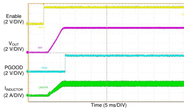
Figure 67. Start-up Waveform
