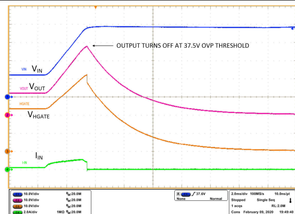
Figure 9-6. Overvoltage Cut-off
