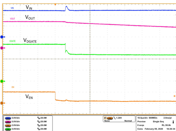
Figure 9-10. Disable Delay DGATE
