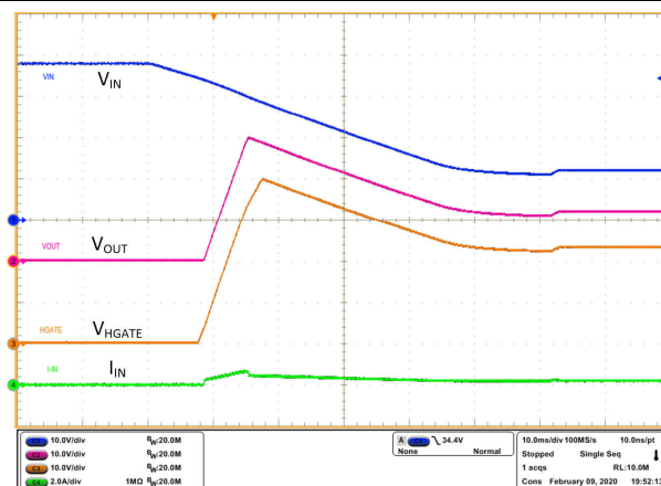
Figure 9-7. Overvoltage Recovery
