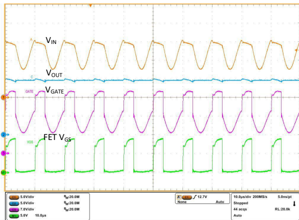
Figure 9-3. AC Super Imposed Test - 6-V Peak-Peak 100 kHz
