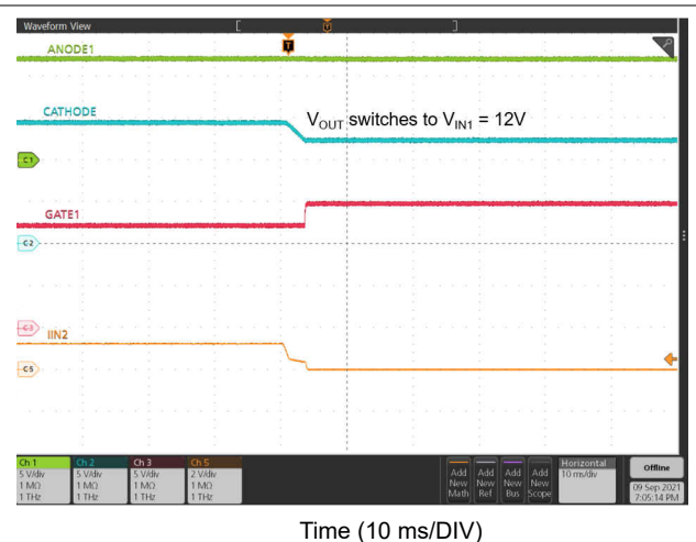
Figure 9-16. ORing V_{IN2} to V_{IN1} Switch Over
