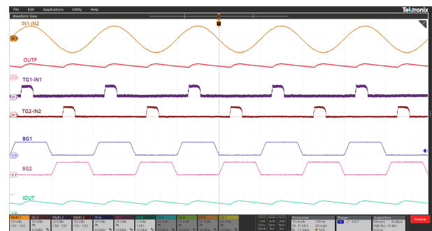
24V AC Input, C_{OUT} = 1\text{mF} , 30W Load, Steady State
