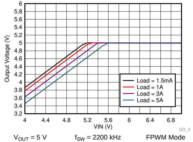
Figure 52. LM73605 Dropout Curve
