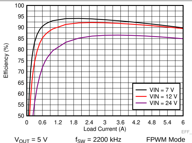
Figure 38. LM73606 Efficiency
