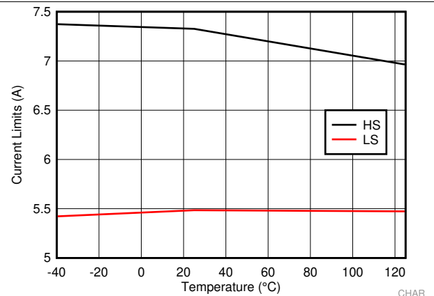
Figure 4. LM73605 High-Side and Low-Side Current Limits
