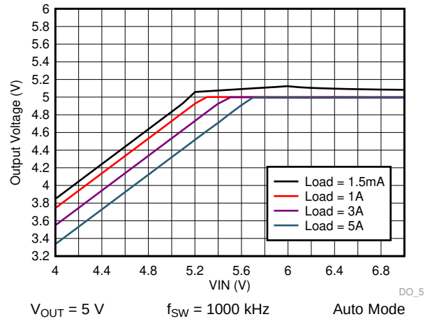
Figure 54. LM73605 Dropout Curve
