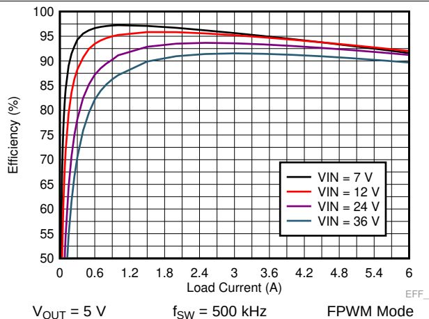
Figure 34. LM73606 Efficiency
