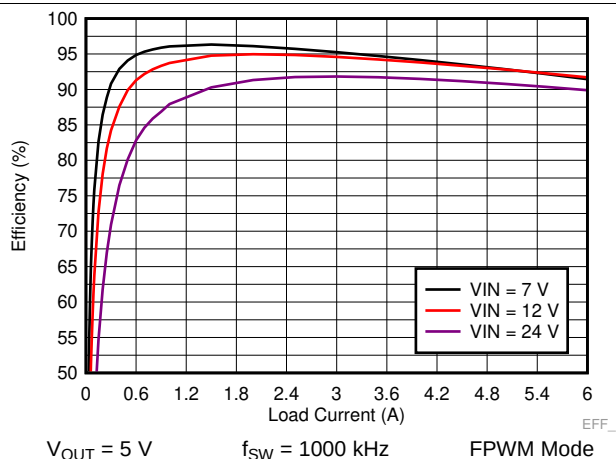
Figure 36. LM73606 Efficiency
