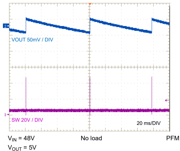
Figure 7-16. PFM Switching
