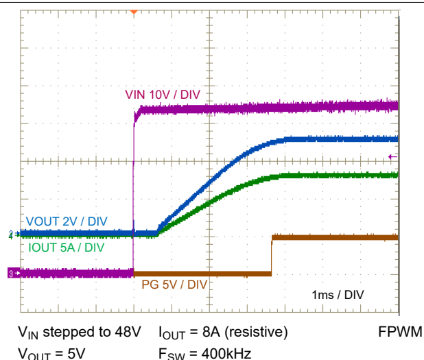
Figure 7-17. Start-Up Characteristic
