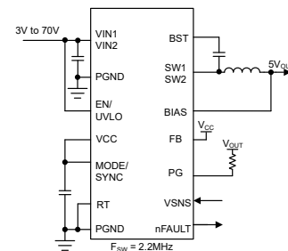
Simplified Schematic
