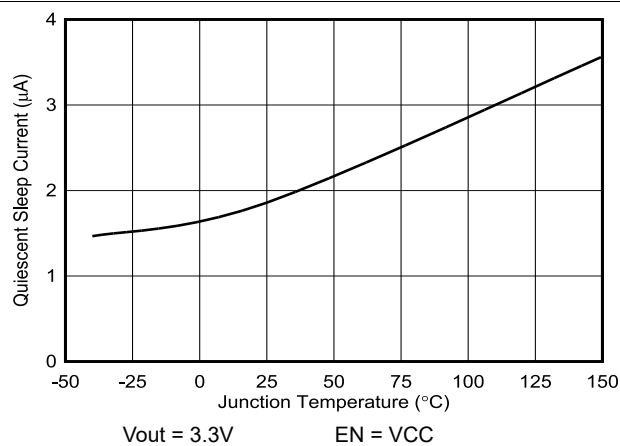
Figure 6-5. Sleep Quiescent Current 3.3V Output
