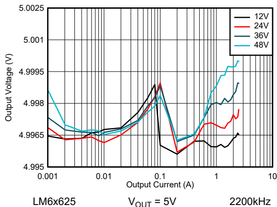
Figure 8-9. LM6xx25 Line and Load Regulation - Auto Mode
