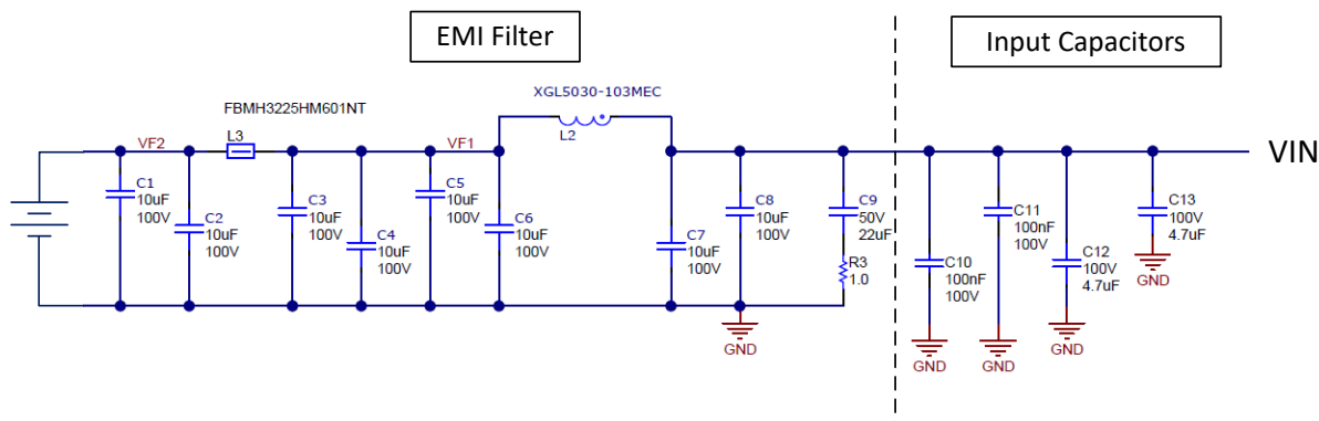
Figure 8-30. EMI Input Filter for 400kHz
