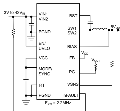
Simplified Schematic
