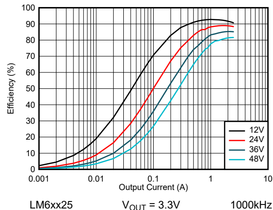
Figure 8-12. LM6xx25 Efficiency - FPWM Mode
