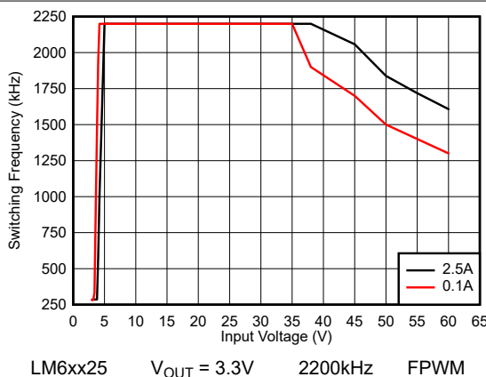
Figure 8-16. LM6xx25 Switching Frequency vs Input Voltage
