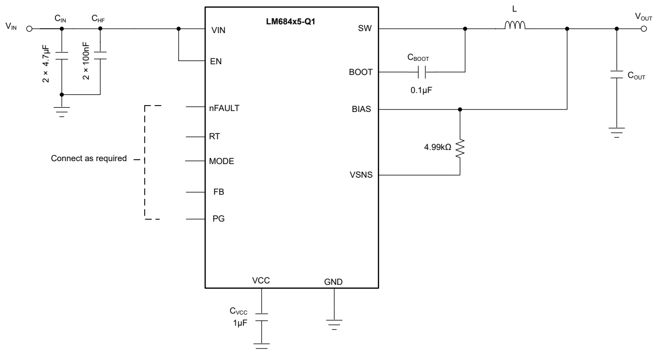
Figure 8-2. Example Application Circuit for Fixed Output Voltage Mode With LM684x5-Q1
