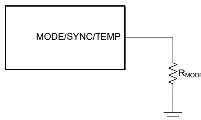
Figure 7-12. Temperature Sensor
