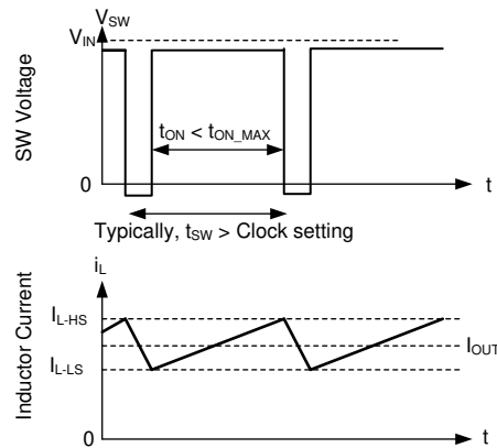
Figure 7-11. Current Limit Waveforms
