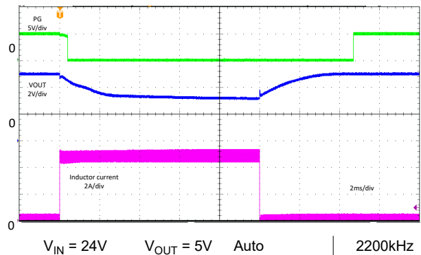
Figure 8-26. Current Limit Transient
