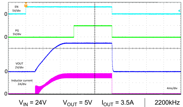
Figure 8-24. Start-Up, Shutdown - FPWM
