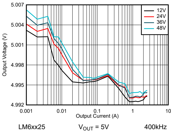
Figure 8-7. LM6xx25 Line and Load Regulation - Auto Mode
