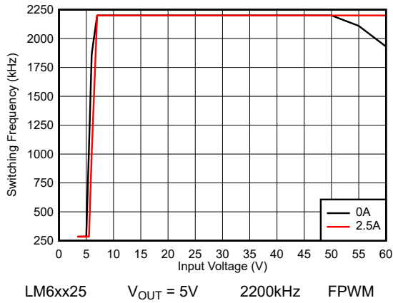
Figure 8-17. LM6xx25 Switching Frequency vs Input Voltage
