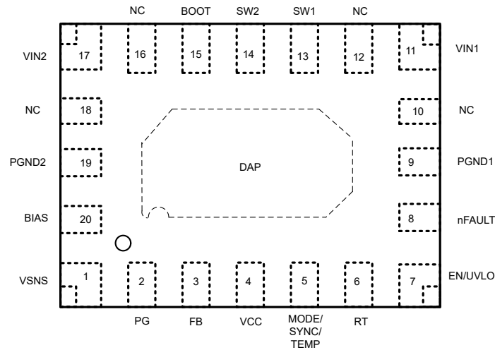
Figure 4-1. 20-Pin RZT, WQFN-FCRLF Package (Top View)
