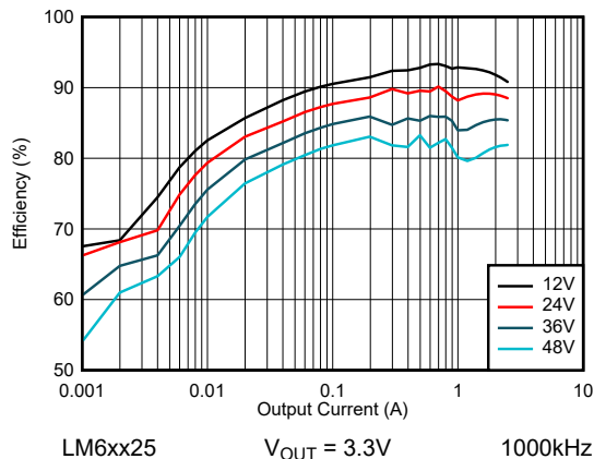
Figure 8-11. LM6xx25 Efficiency - Auto Mode
