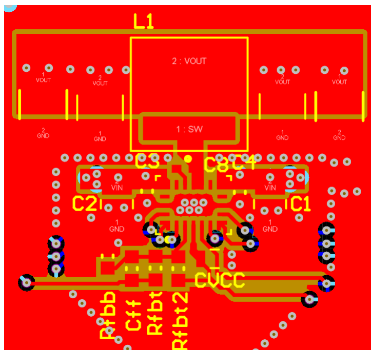
Figure 8-32. Layout Example
