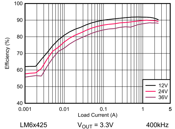
Figure 8-6. LM6x425 Efficiency - Auto Mode
