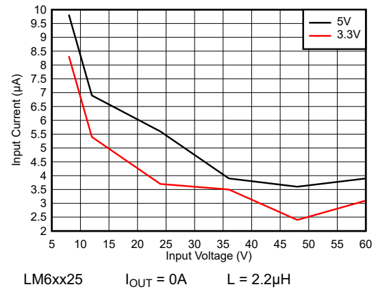
Figure 8-20. No Load Input Supply Current - Auto Mode
