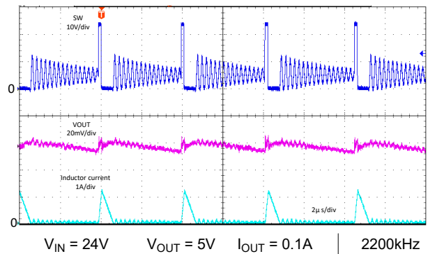
Figure 8-22. Typical Switching Waveforms - LM6xx25 - Auto
