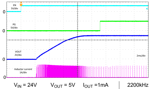
Figure 8-23. Start-Up - Auto
