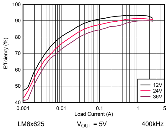
Figure 6-1. LM6x625 Efficiency - Auto Mode
