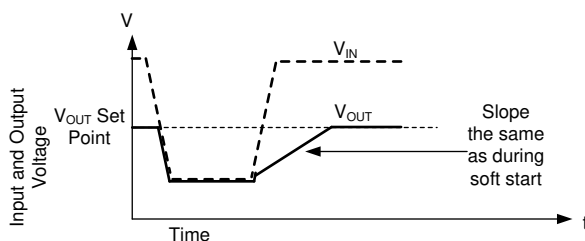
Figure 7-18. When Output Voltage Falls, Output Voltage Recovers Slowly, Preventing Overshoot and Large Inrush Currents
