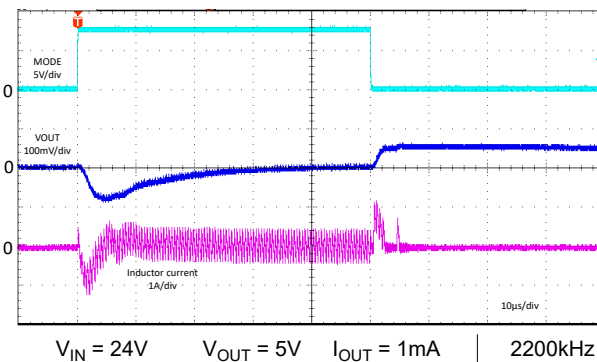
Figure 8-27. MODE Change Transient
