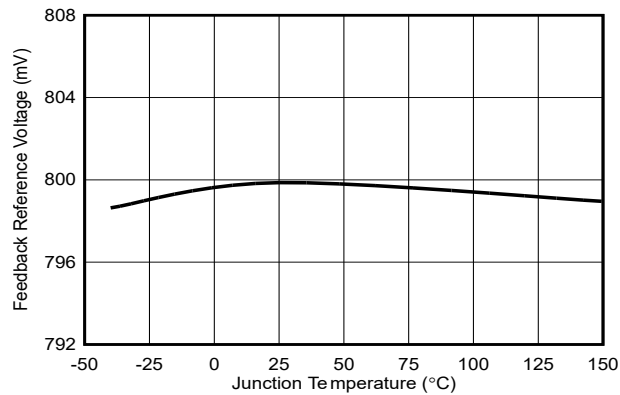
Figure 6-3. Feedback Voltage
