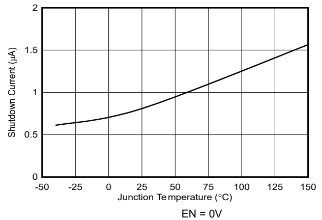
Figure 6-4. Shutdown Input Current
