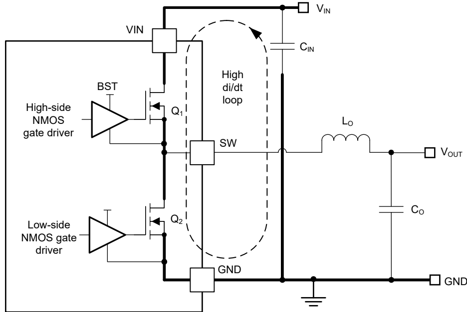
Figure 8-31. Current Loops With Fast Edges
