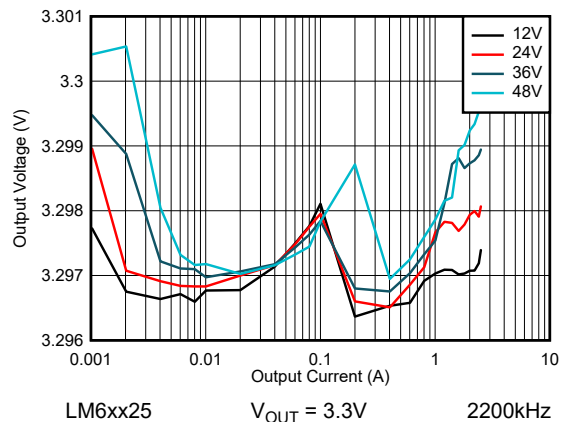
Figure 8-10. LM6xx25 Line and Load Regulation - Auto Mode
