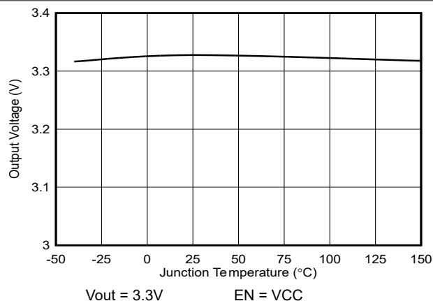
Figure 6-7. Fixed 3.3V Output
