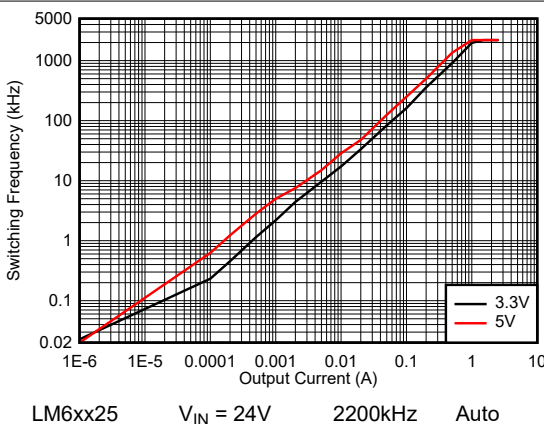
Figure 8-15. LM6xx25 Switching Frequency vs Load Current
