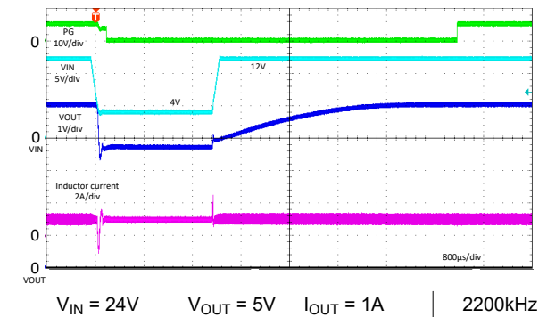
Figure 8-28. Dropout Transient and Recovery
