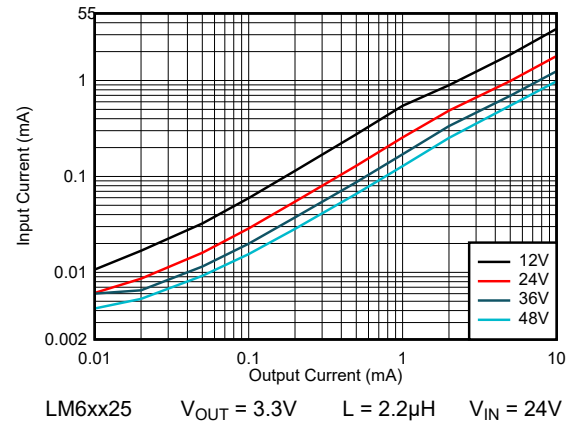
Figure 8-18. Input Supply Current - Auto Mode
