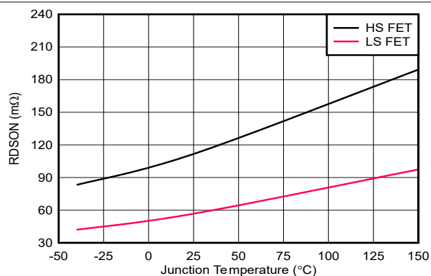
Figure 6-10. LS and HS FET RDSON
