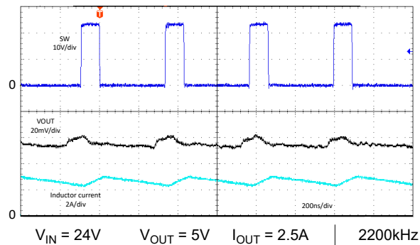
Figure 8-21. Typical Switching Waveforms - LM6xx25 - FPWM
