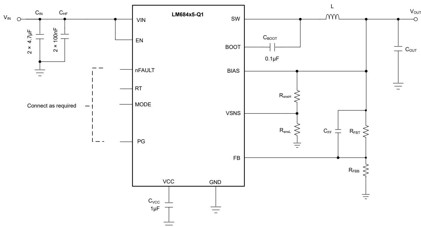
Figure 8-1. Example Application Circuit for Adjustable Output Voltage Mode With LM684x5-Q1
