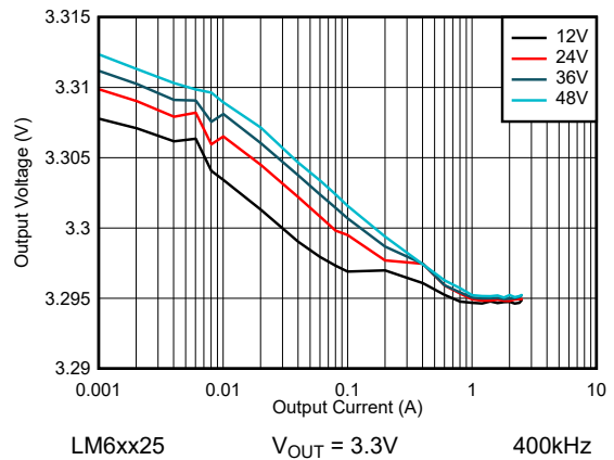
Figure 8-8. LM6xx25 Line and Load Regulation - Auto Mode
