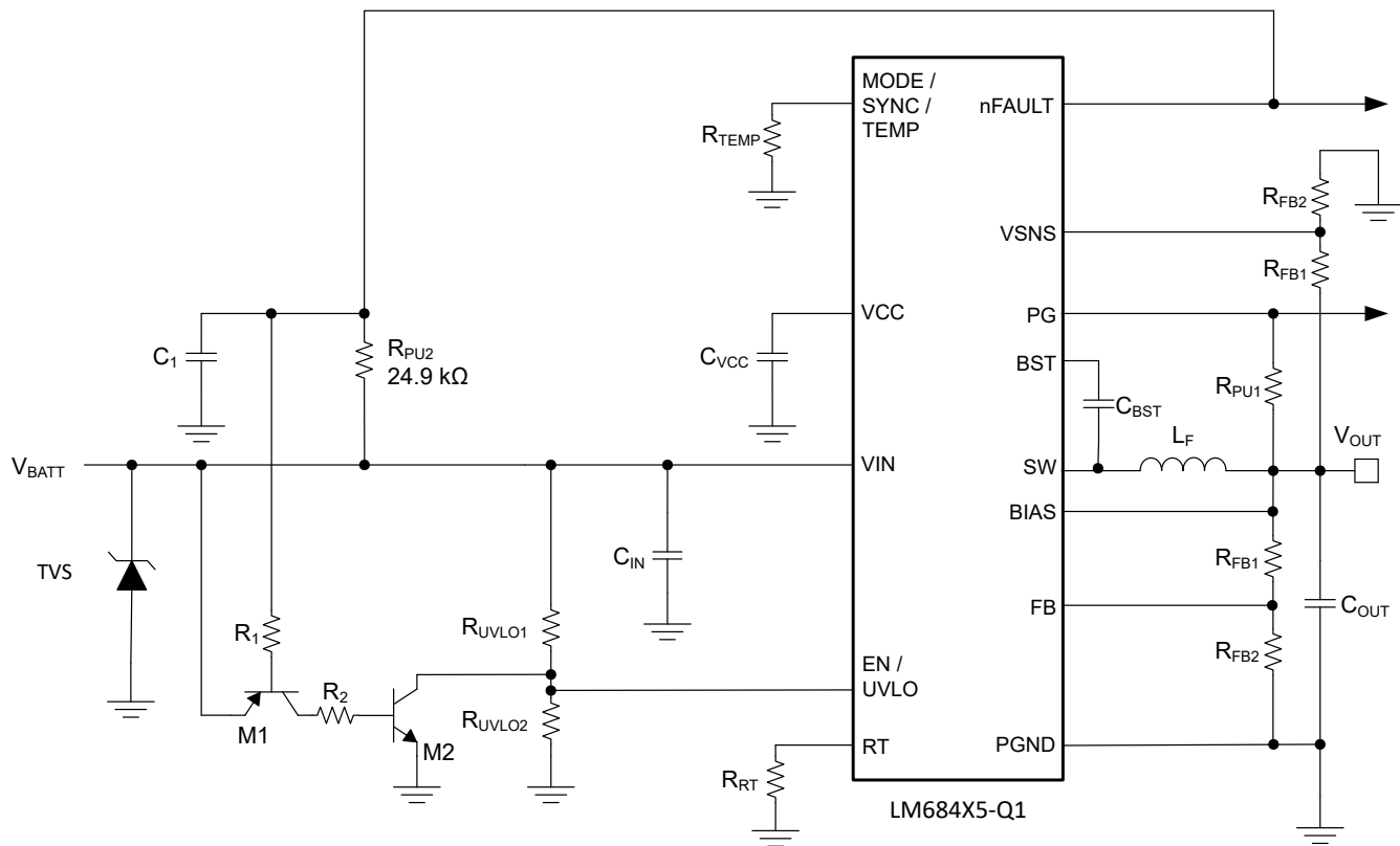
Figure 7-10. Redundant Monitoring of an Adjustable VOUT With an Auto-Retry Scheme
