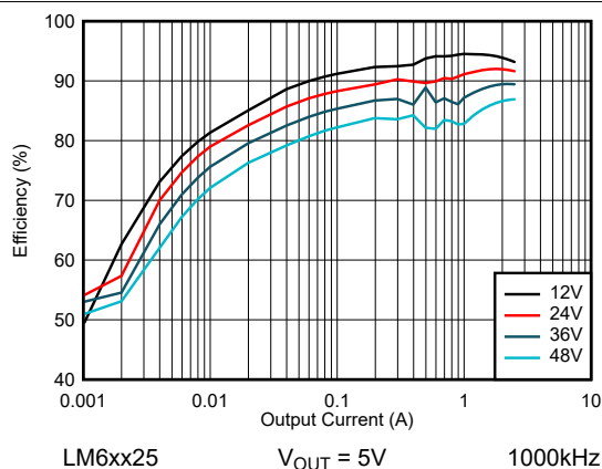
Figure 8-13. LM6xx25 Efficiency - Auto Mode
