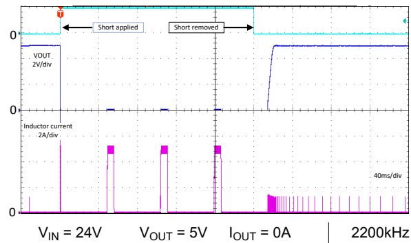
Figure 8-25. Output Short Circuit and Recovery - Auto
