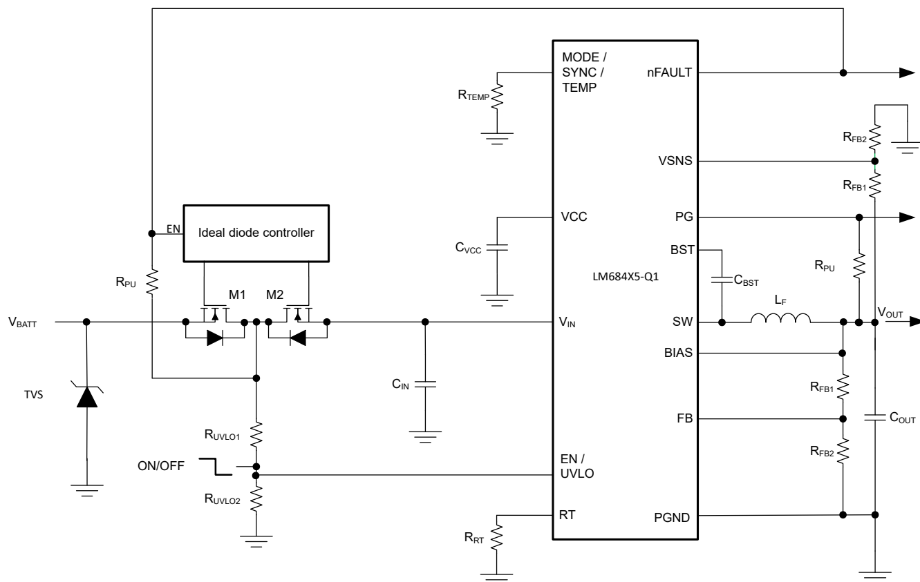
Figure 7-9. Redundant Monitoring of an Adjustable V_{OUT}
