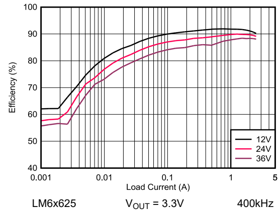
Figure 6-2. LM6x625 Efficiency - Auto Mode
