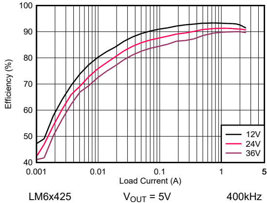
Figure 8-5. LM6x425 Efficiency - Auto Mode
