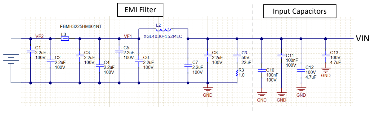
Figure 8-29. EMI Input Filter for 2200kHz
