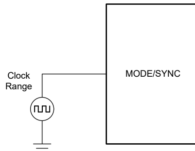
Figure 7-3. Typical Implementation Allowing Synchronization Using the MODE/SYNC/TEMP Pin
