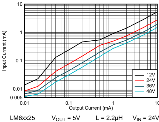
Figure 8-19. Input Supply Current - Auto Mode
