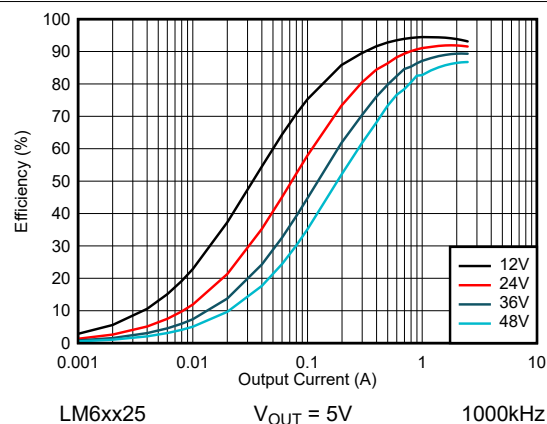
Figure 8-14. LM6xx25 Efficiency - FPWM Mode
