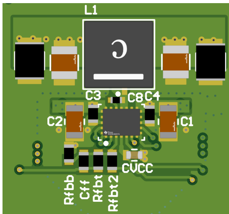
Figure 8-33. PCB Image
