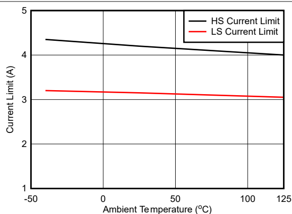
Figure 6-9. 2.5A Current Limit
