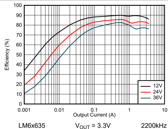
Figure 8-14. LM6x635 Efficiency - Auto Mode
