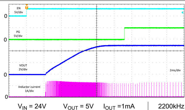
Figure 8-87. Start-Up - Auto
