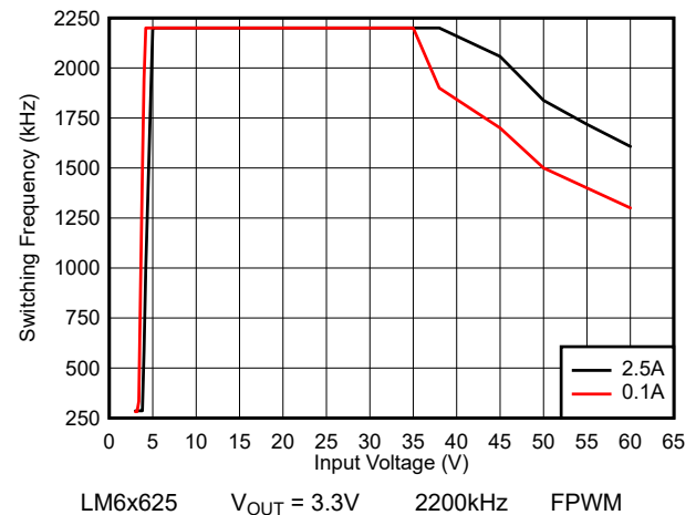
Figure 8-58. LM6x625 Switching Frequency vs Input Voltage
