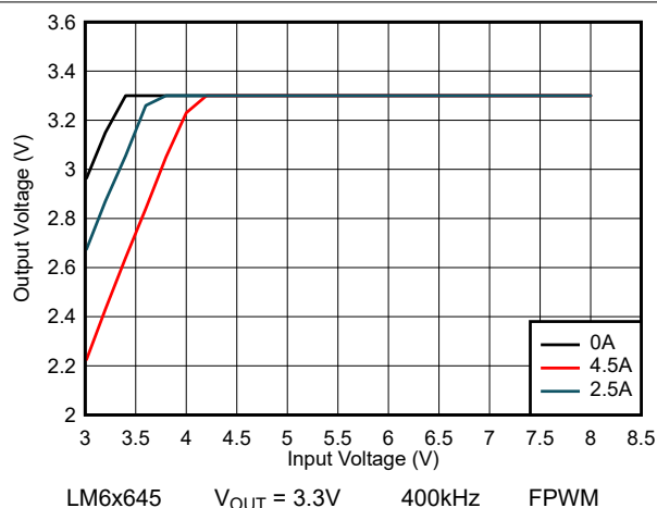
Figure 8-63. LM6x645 Dropout Characteristic
