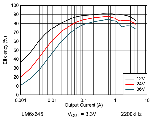
Figure 8-18. LM6x645 Efficiency - Auto Mode
