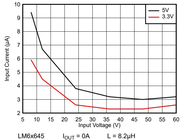
Figure 8-74. No Load Input Supply Current - Auto Mode
