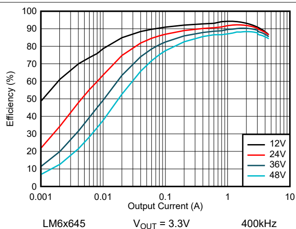
Figure 8-16. LM6x645 Efficiency - Auto Mode
