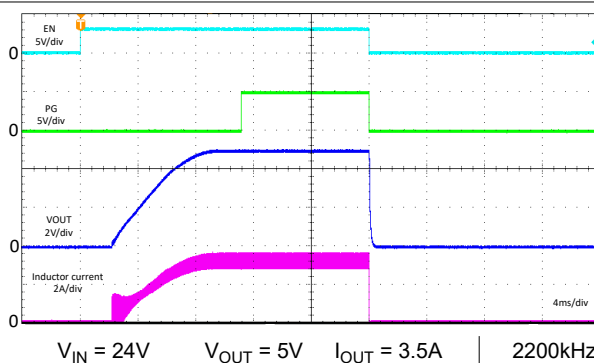
Figure 8-88. Start-Up, Shutdown - FPWM
