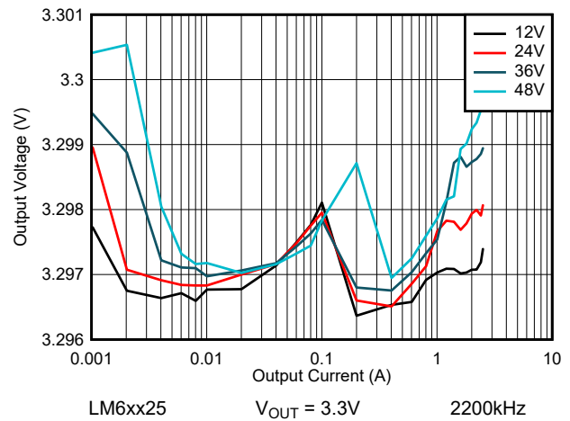
Figure 8-22. LM6xx25 Line and Load Regulation - Auto Mode
