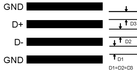
Figure 9-1. Ideal Diode Trace Layout
