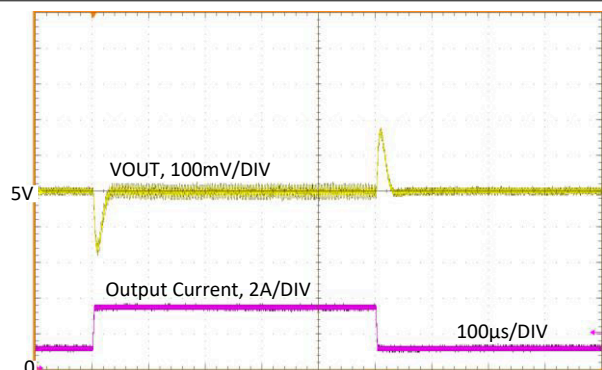
Figure 8-19. Load Transient
