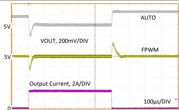
Figure 8-17. Load Transient
