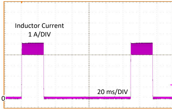
Figure 7-11. Inductor Current Burst in Short-Circuit Mode
