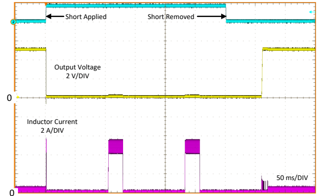
Figure 7-12. Short-Circuit Transient and Recovery
