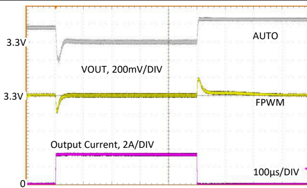
Figure 8-18. Load Transient
