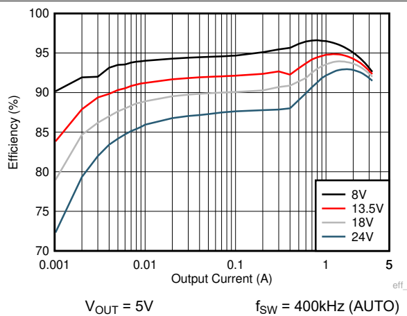
Figure 8-7. Efficiency
