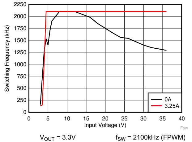
Figure 8-15. Switching Frequency vs Input Voltage
