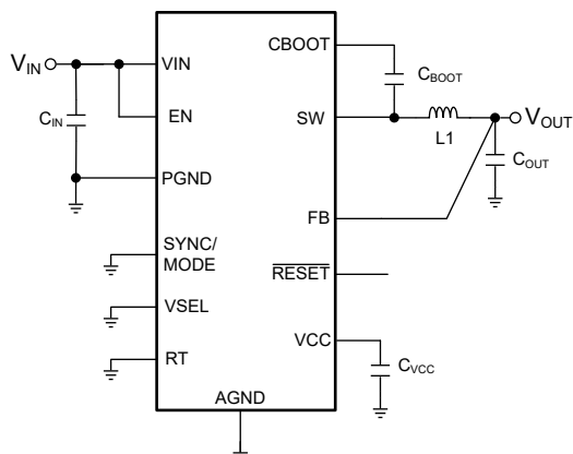
Simplified Schematic
