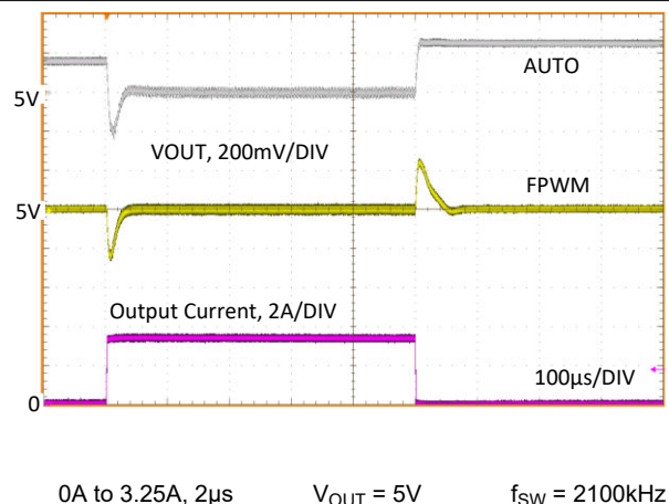
Figure 8-22. Load Transient
