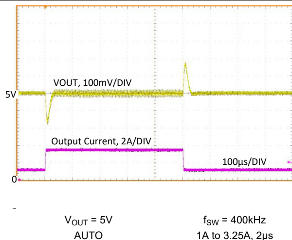
Figure 8-24. Load Transient
