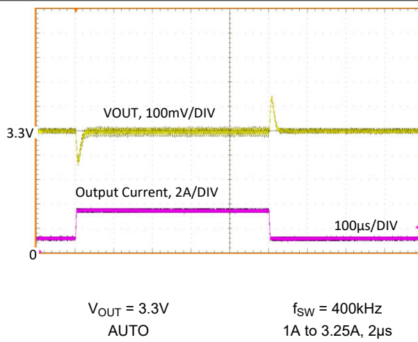
Figure 8-25. Load Transient
