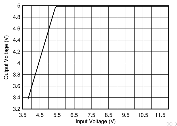
Figure 7-11. Overall Dropout Characteristic V_{OUT} = 5V , I_{OUT} = 3.25A
