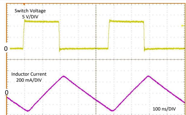
Figure 7-7. Typical PWM Switching Waveforms Without Spread Spectrum V_{IN} = 12V , V_{OUT} = 5V , I_{OUT} = 3.25A , f_{SW} = 2100kHz
