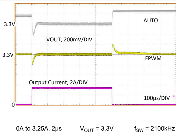
Figure 8-23. Load Transient
