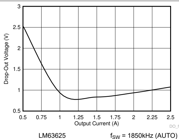
Figure 8-35. Dropout Voltage versus Output Current to 1.85MHz
