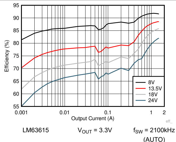
Figure 8-15. Efficiency
