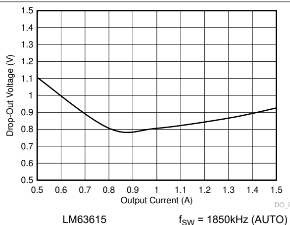
Figure 8-37. Dropout Voltage versus Output Current to 1.85MHz
