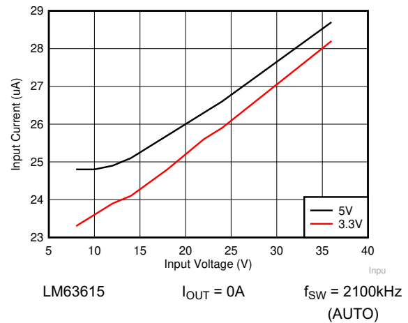
Figure 8-39. Input Supply Current versus Input Voltage
