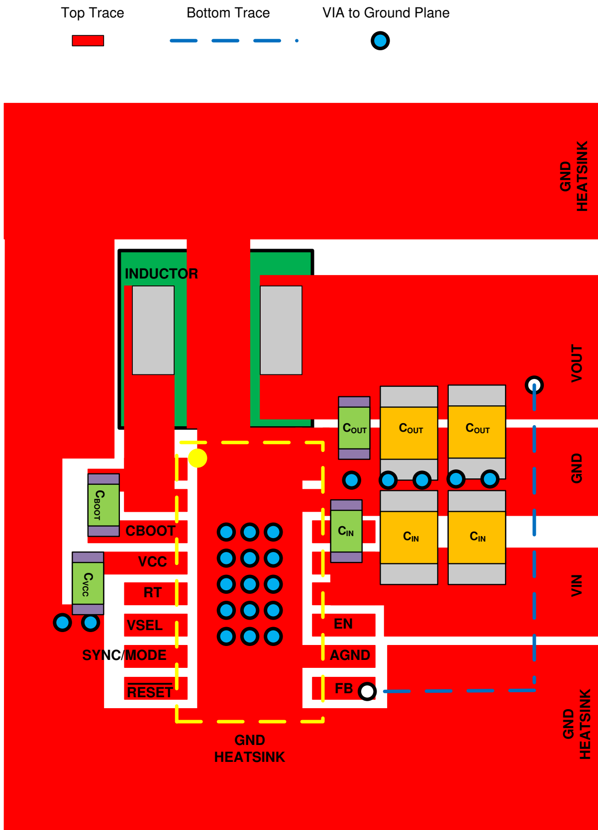
Figure 8-49. Example Layout for HTSSOP Package
