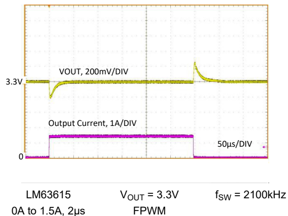
Figure 8-27. Load Transient
