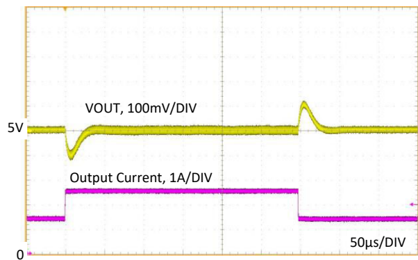
LM63625 V_{OUT} = 5V f_{SW} = 2100kHz 1.5A to 2.5A, 2µs AUTO
