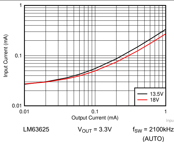
Figure 8-42. Input Supply Current versus Output Current
