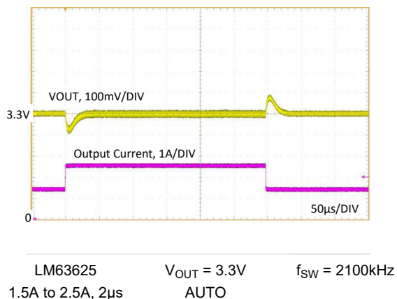
Figure 8-30. Load Transient
