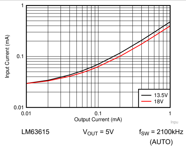
Figure 8-41. Input Supply Current versus Output Current
