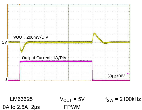
Figure 8-28. Load Transient
