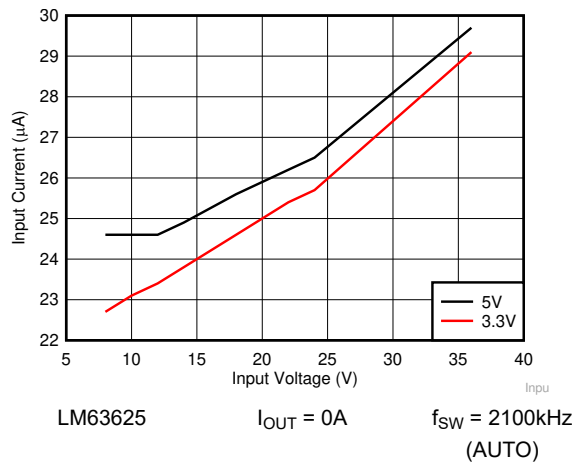
Figure 8-38. Input Supply Current versus Input Voltage
