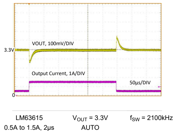
Figure 8-31. Load Transient
