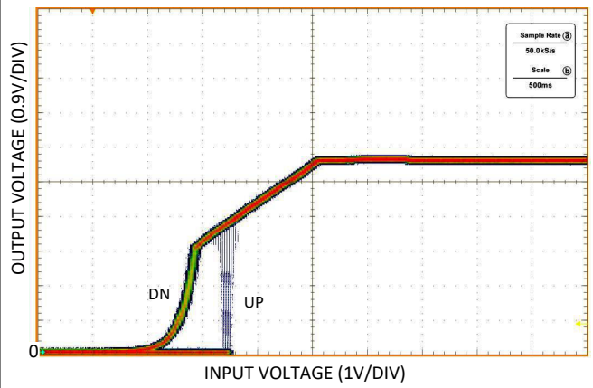
Figure 6-2. UVLO Thresholds
