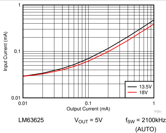
Figure 8-40. Input Supply Current versus Output Current
