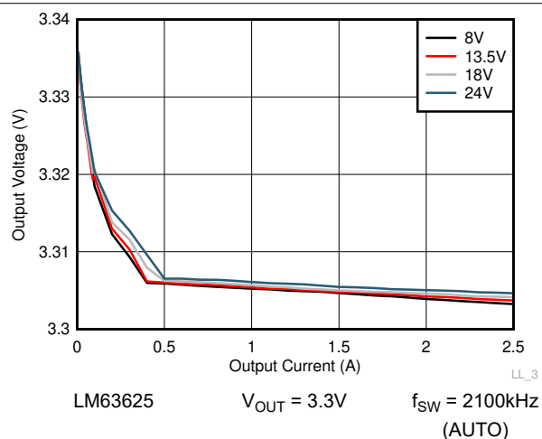
Figure 8-17. Line and Load Regulation
