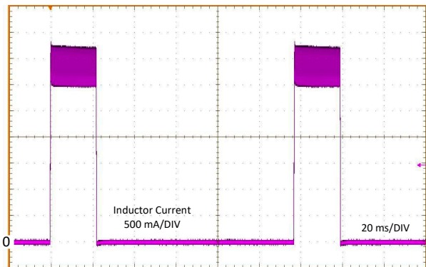
Figure 7-12. Inductor Current Burst in Short-Circuit Mode; LM63625
