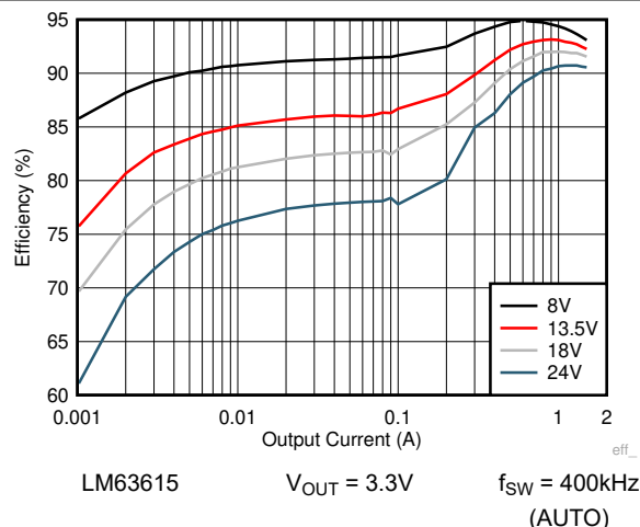
Figure 8-14. Efficiency
