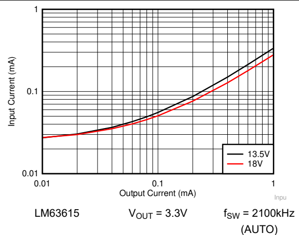
Figure 8-43. Input Supply Current versus Output Current
