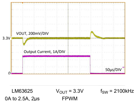
Figure 8-26. Load Transient
