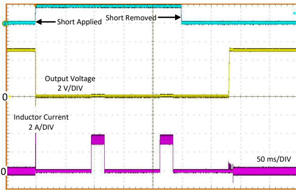
Figure 7-13. Short-Circuit Transient and Recovery; LM63625
