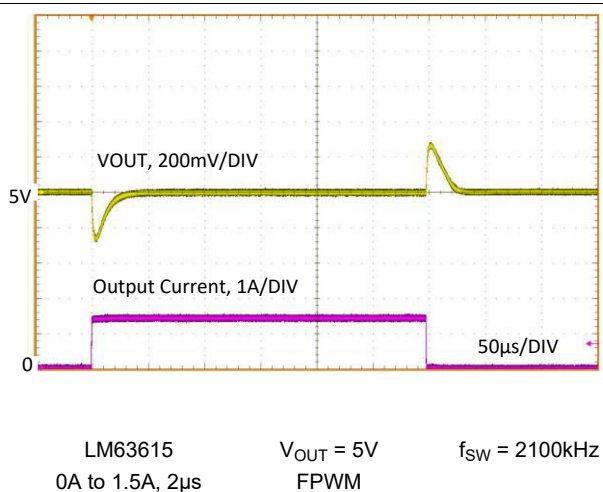
Figure 8-29. Load Transient
