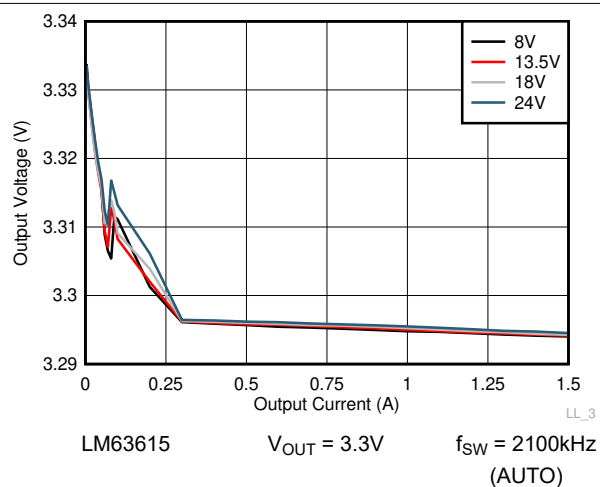
Figure 8-19. Line and Load Regulation
