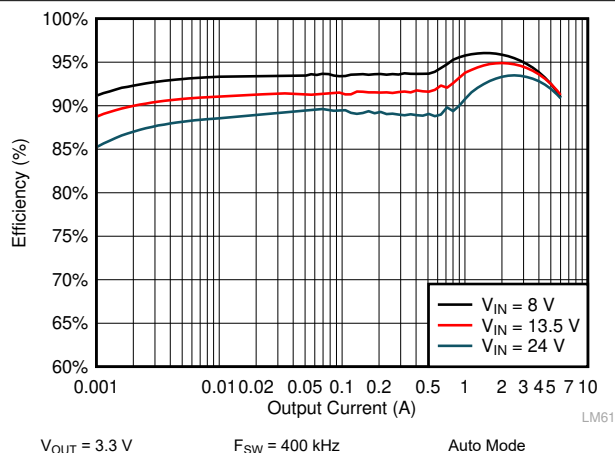
Figure 10-5. LM61460-Q1 Efficiency
