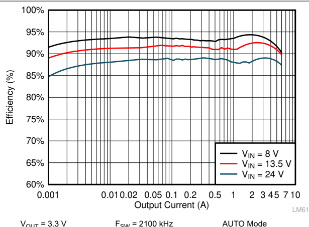
Figure 10-7. LM61460-Q1 Efficiency
