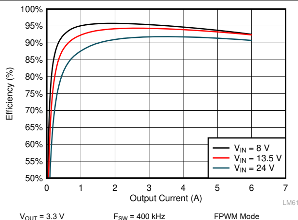
Figure 10-6. LM61460-Q1 Efficiency
