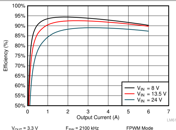
Figure 10-8. LM61460-Q1 Efficiency
