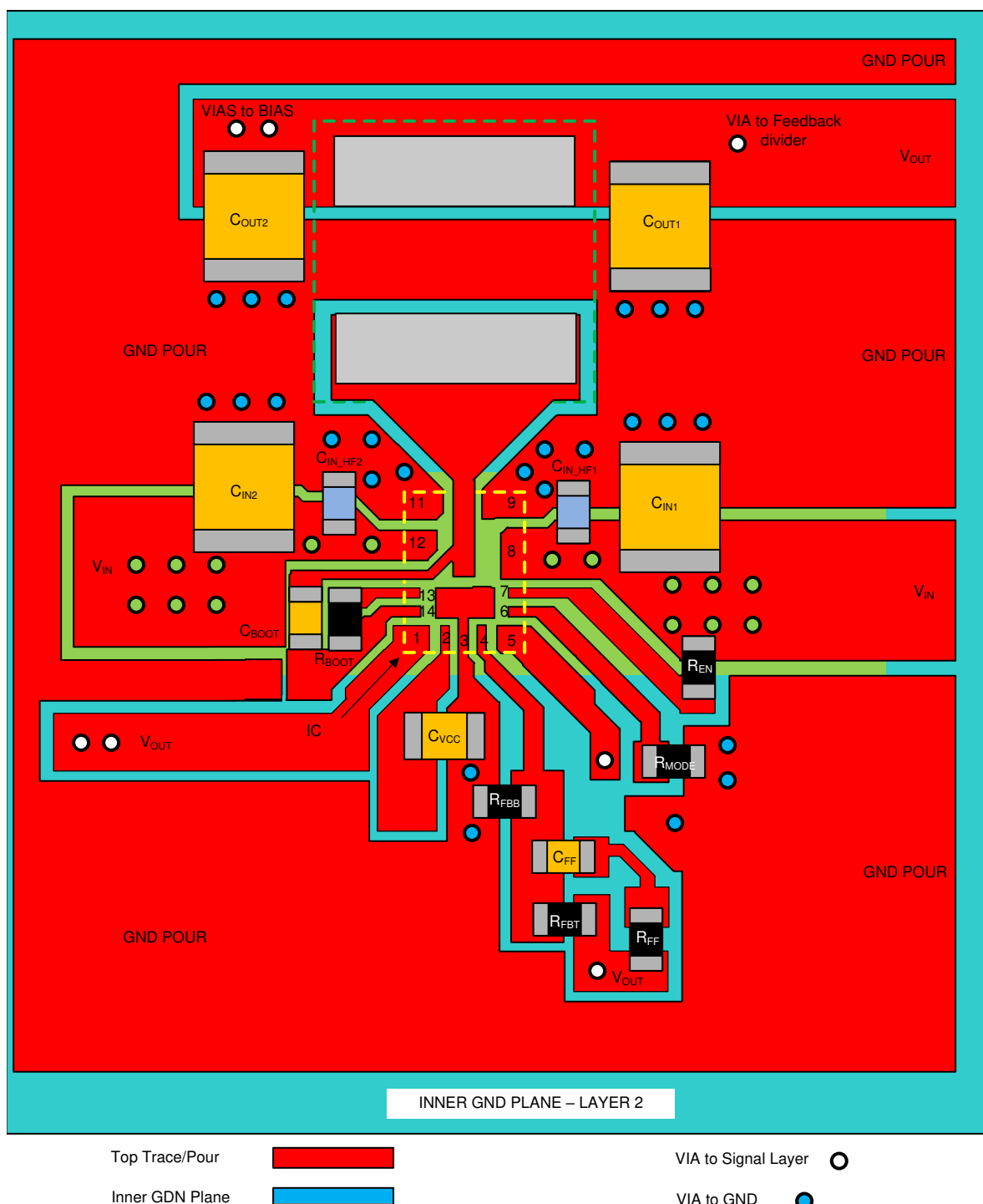
Figure 12-2. Layout Example
