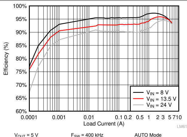
Figure 10-9. LM61460-Q1 Efficiency
