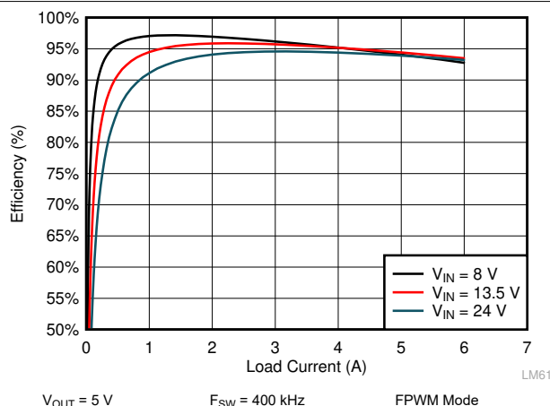
Figure 10-10. LM61460-Q1 Efficiency
