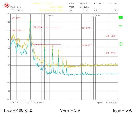
Figure 9-54. Conducted EMI versus CISPR25 Limits (Yellow: Peak Signal, Blue: Average Signal)
