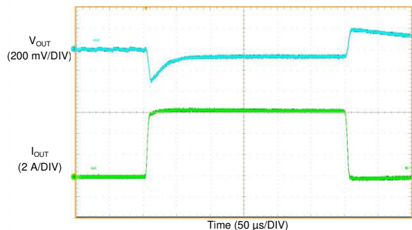
Figure 9-47. LM61460 Load Transient
