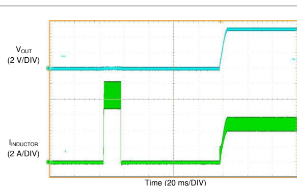
Figure 8-15. Short-Circuit Recovery
