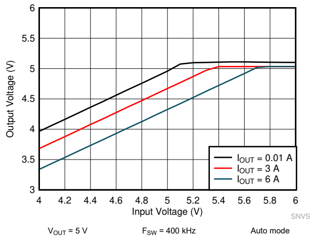
Figure 9-31. Dropout Curve
