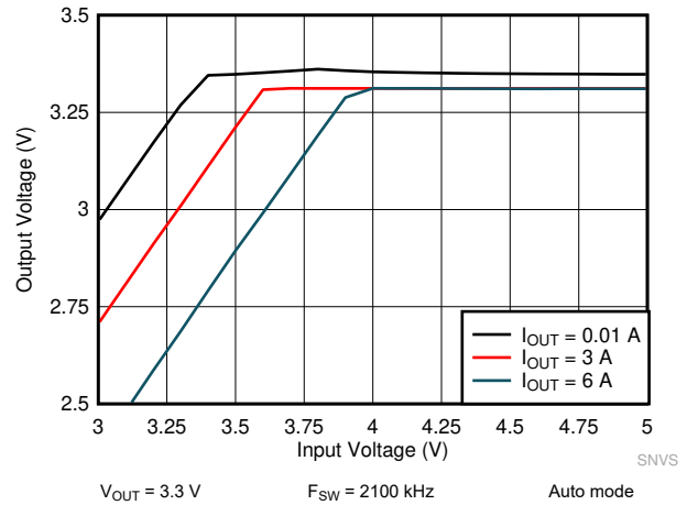
Figure 9-30. LM61460 Dropout Curve
