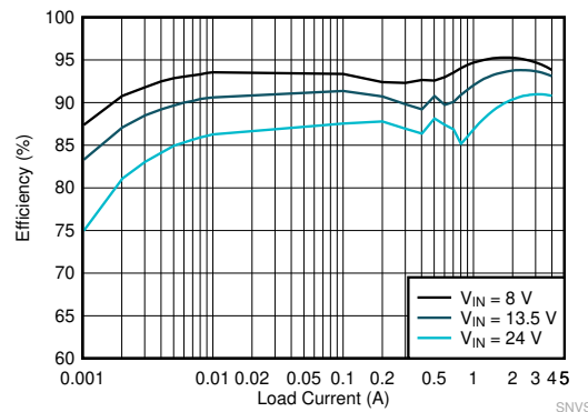
Efficiency V_{\text{OUT}} = 5 \text{ V} , f_{\text{SW}} = 2200 \text{ kHz}
