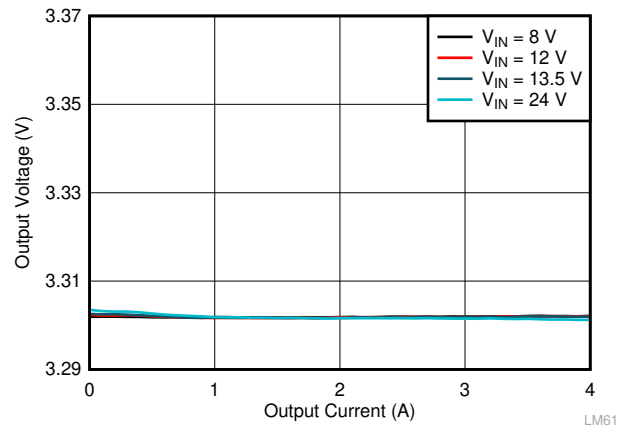
Figure 10-12. LM61440-Q1 Load and Line Regulation
