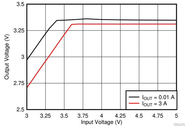
Figure 10-18. LM61440-Q1 Dropout Curve
