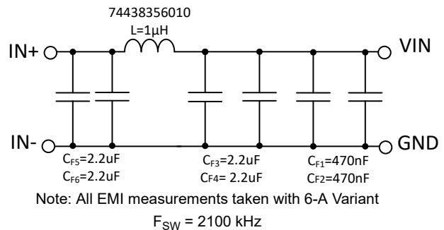
Figure 10-44. Recommended Input EMI Filter
