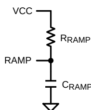
Figure 13. R_{RAMP} to V_{CC} for V_{OUT} > 7.5 V
