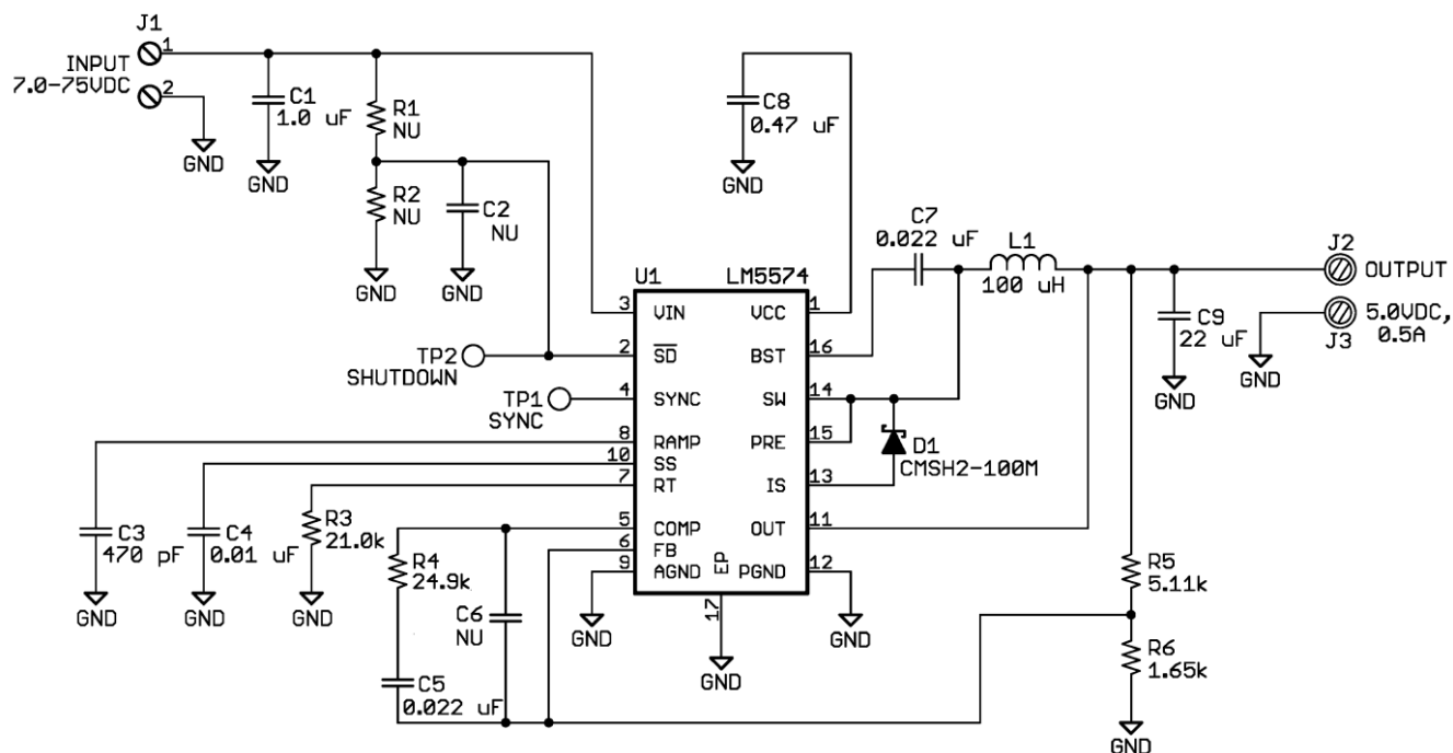
Figure 7-3. Typical Application Schematic
