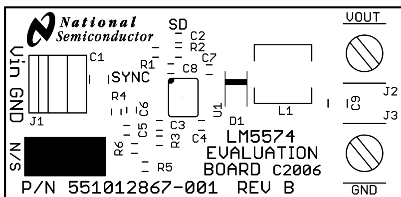
Figure 7-14. Silkscreen
