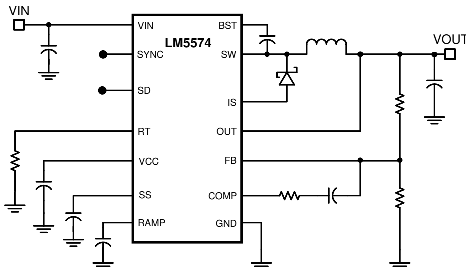
Simplified Application Schematic
