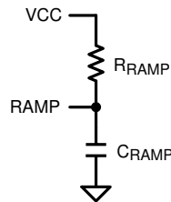
Figure 6-6. R RAMP to V CC for V OUT > 7.5V
