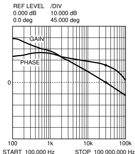
Figure 7-7. Overall Loop Gain and Phase
