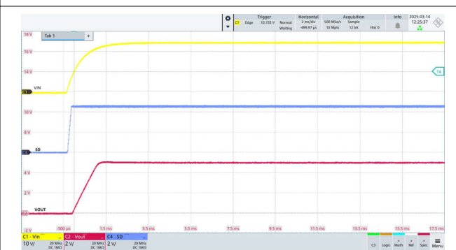
Figure 7-11. Start-Up Operation
