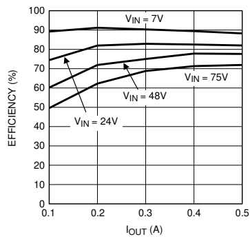
Figure 5-7. Demoboard Efficiency vs IOUT and VIN
