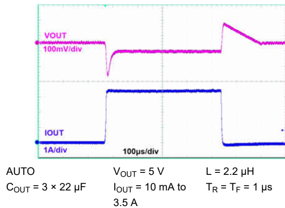
Figure 9-16. Load Transients
