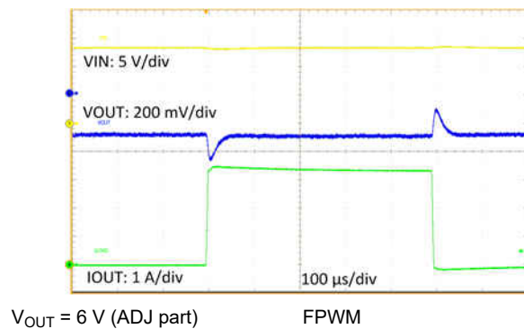
Figure 9-38. Load Transient
