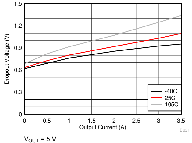
Figure 9-12. Dropout for \geq 1.85\text{ MHz}
