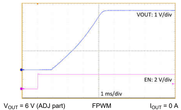
Figure 9-36. Start-up Waveform
