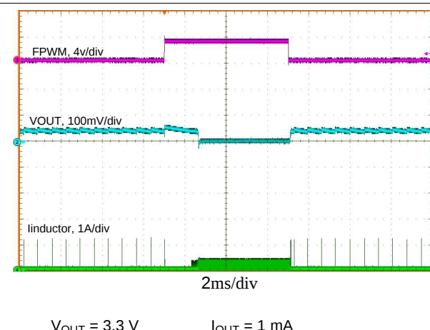
Figure 44. Mode Change Transient
