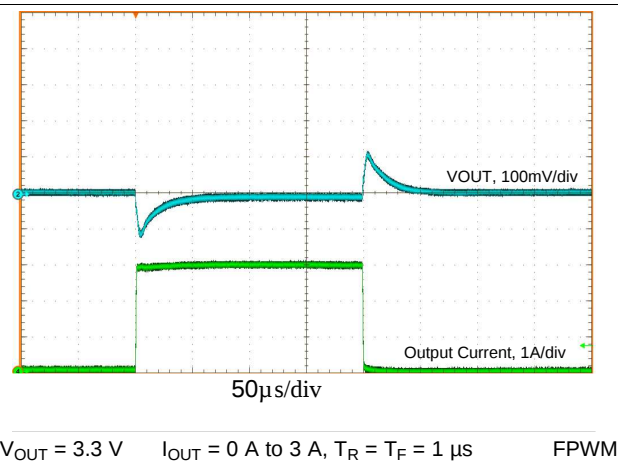
Figure 43. Load Transient
