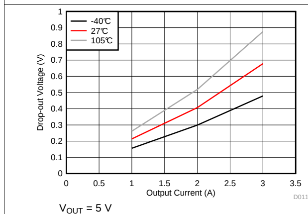
Figure 25. Dropout for -1% Regulation
