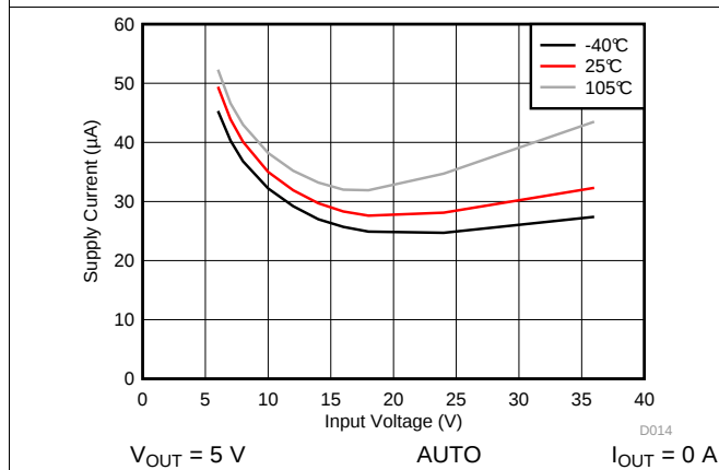
Figure 23. Input Supply Current
