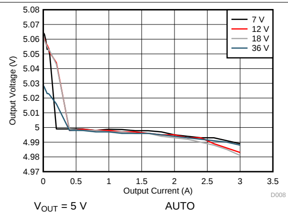
Figure 22. Load and Line Regulation
