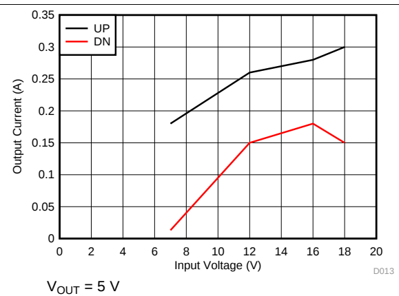
Figure 24. Load Current for Mode Change
