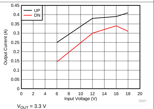
Figure 36. Load Current for Mode Change
