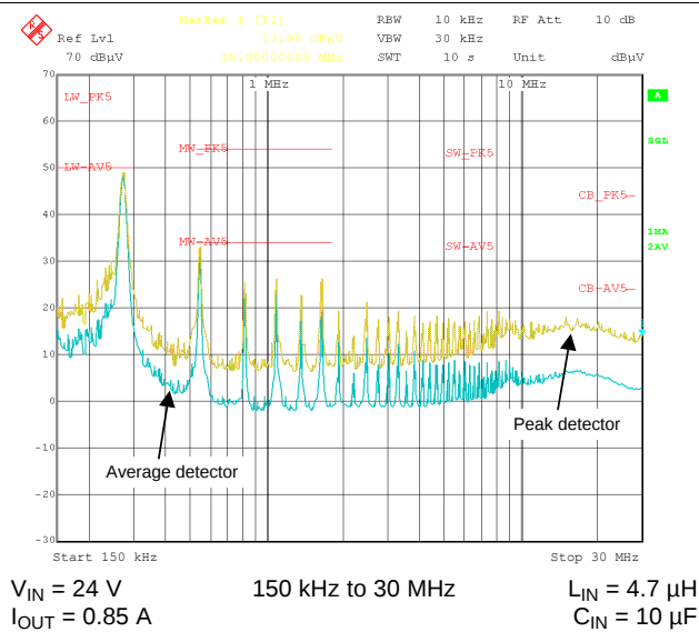
Figure 36. CISPR 25 Class 5 Conducted EMI Plot
