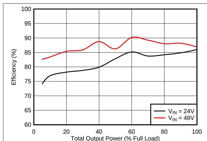
Figure 52. Efficiency
