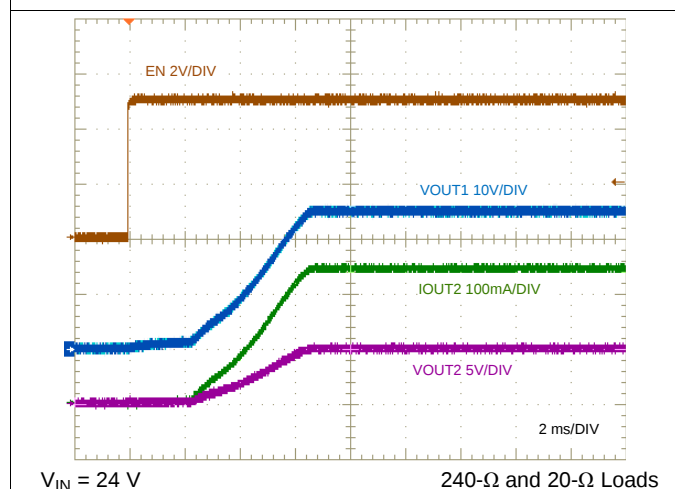
Figure 54. ENABLE ON Characteristic
