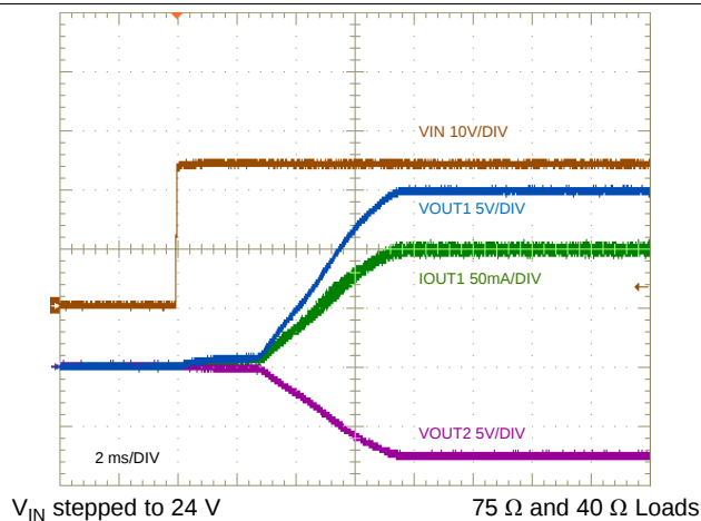
Figure 43. Start-Up Characteristic
