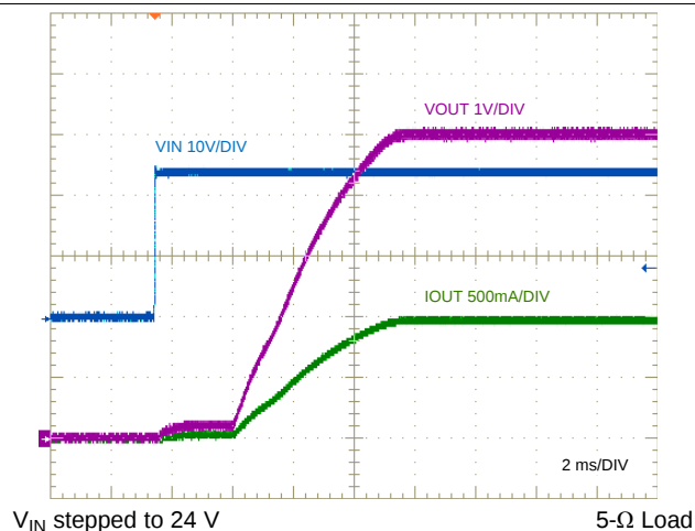
Figure 29. Start-up Characteristic
