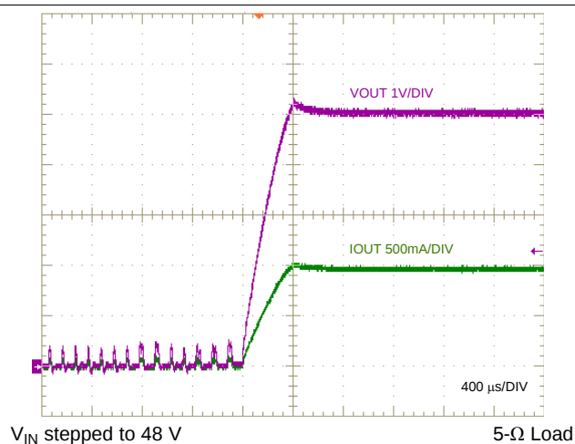
Figure 31. Short Circuit Recovery
