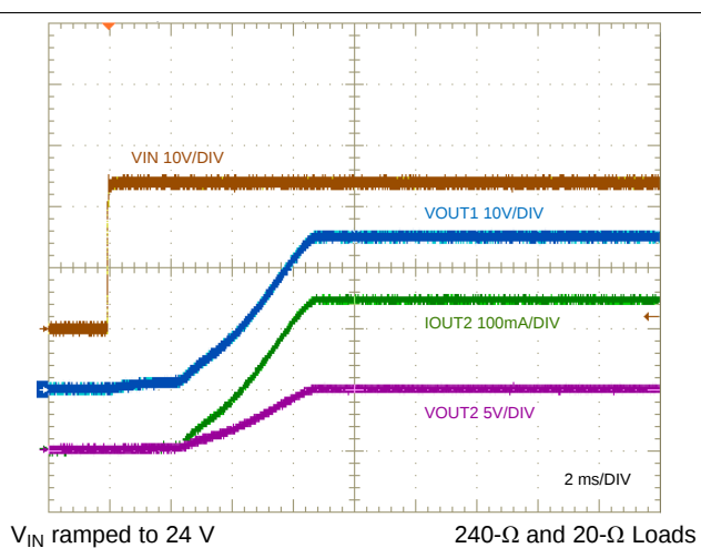
Figure 53. Start-Up Characteristic
