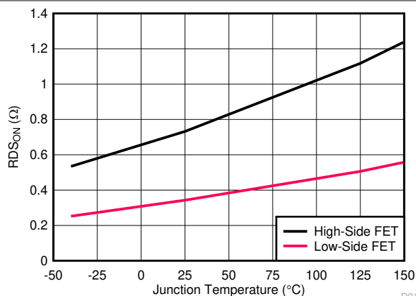
Figure 5-8. MOSFETs On-State Resistance versus Temperature
