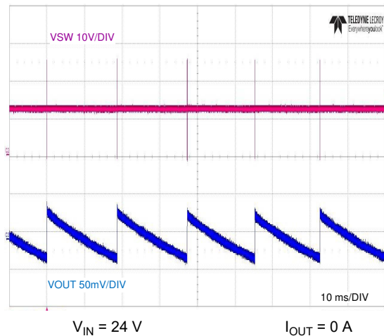
Figure 7-14. No-Load Switching
